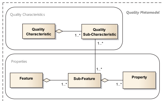
Figure 1: Quality Metamodel.
