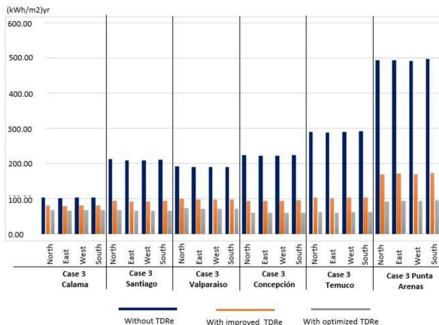
Figure 5. Energy demand for Case 3.
