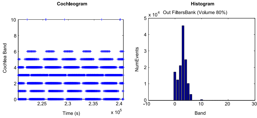
Fig. 7. Response of the spiking digital cochlea to a 689 Hz sine wave.
