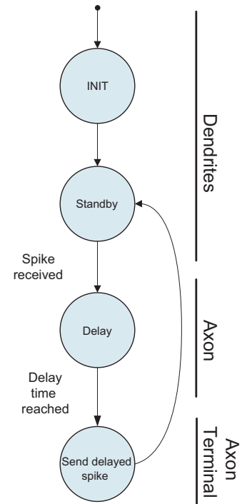
Fig. 12. DelayNeuron finite states machine.
