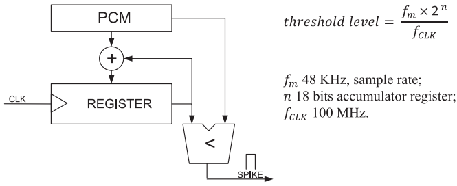
Fig. 5. Accumulator spiking neuron model.
