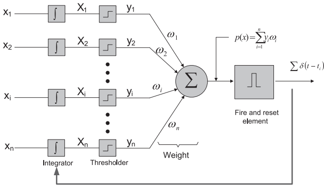
Fig. 8. RNeuron model.
