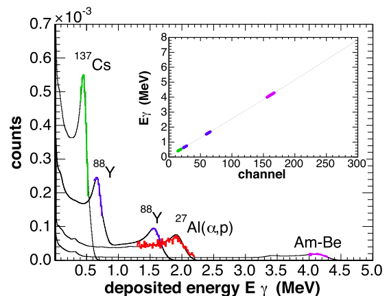
FIG. 5. (Color online) The simulated detector responses and measured spectra from calibration sources. The resulting energy calibration is shown in the inset. The highlighted regions correspond to the intervals where the calibration sources were fitted.
