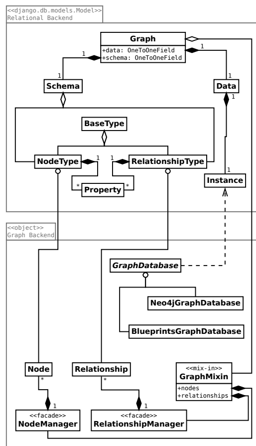
Figure 2: Simplified UML Diagram.
