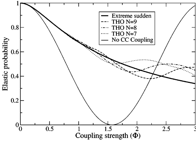
FIG. 3. Ground-state probability in the sudden limit as a function of the parameter \Phi (dimensionless). The thick full line is the full sudden result. The dashed lines correspond to the THO discretization, for several numbers of states. The thin full line is the sudden calculation excluding continuum-to-continuum coupling.
