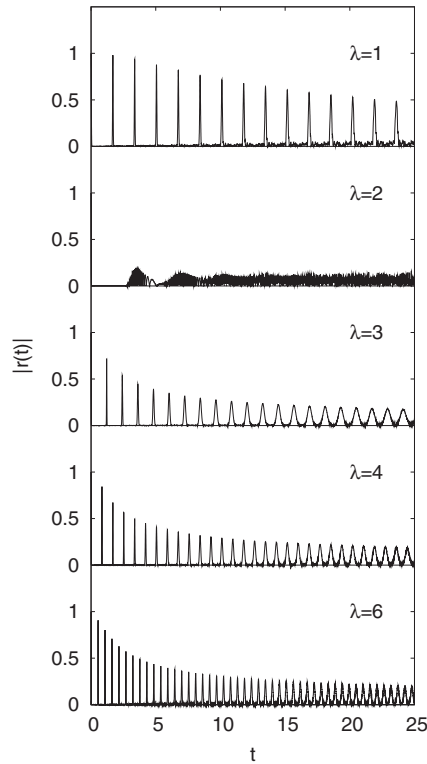
FIG. 2. |r(t)| for \alpha=0 and five different values of \lambda . In all cases N=10\,000 .
