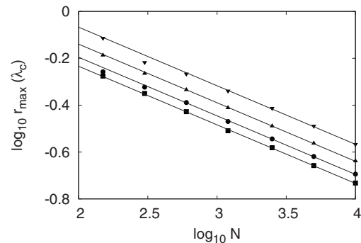
FIG. 4. r_{max}(\lambda_c) in function of the size of the environment N , in a double logarithmic scale. Squares represent the case \alpha=0 ; circles, \alpha=0.4 ; upper triangles, \alpha=0.6 ; lower triangles, \alpha=0.7 . The straight lines correspond to a least squares fit to the power law r_{max}(\lambda_c) = AN^{-1/4} .
