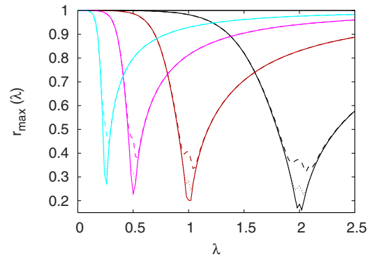
FIG. 3. (Color online) r_{max}(\lambda) in function of the coupling \lambda , for different values of \alpha and N . Black lines represent the case \alpha=0 ; dark gray (red online) lines, \alpha=0.4 ; gray (magenta online), \alpha=0.6 ; and light gray (cyan online), \alpha=0.7 . Solid lines represent N=10\,000 ; dotted lines, N=2500 ; and dashed lines, N=600 .
