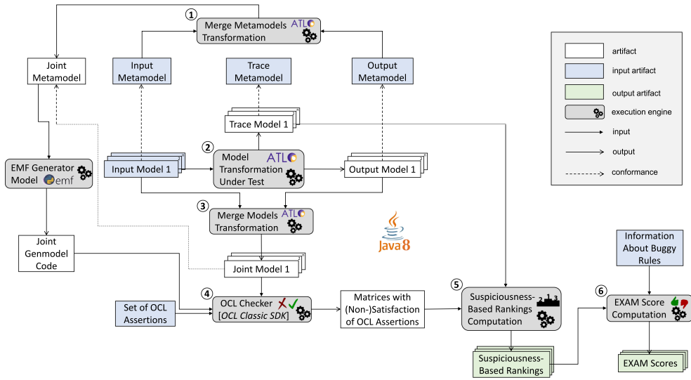
Fig. 5. Implementation and automation of our approach.
