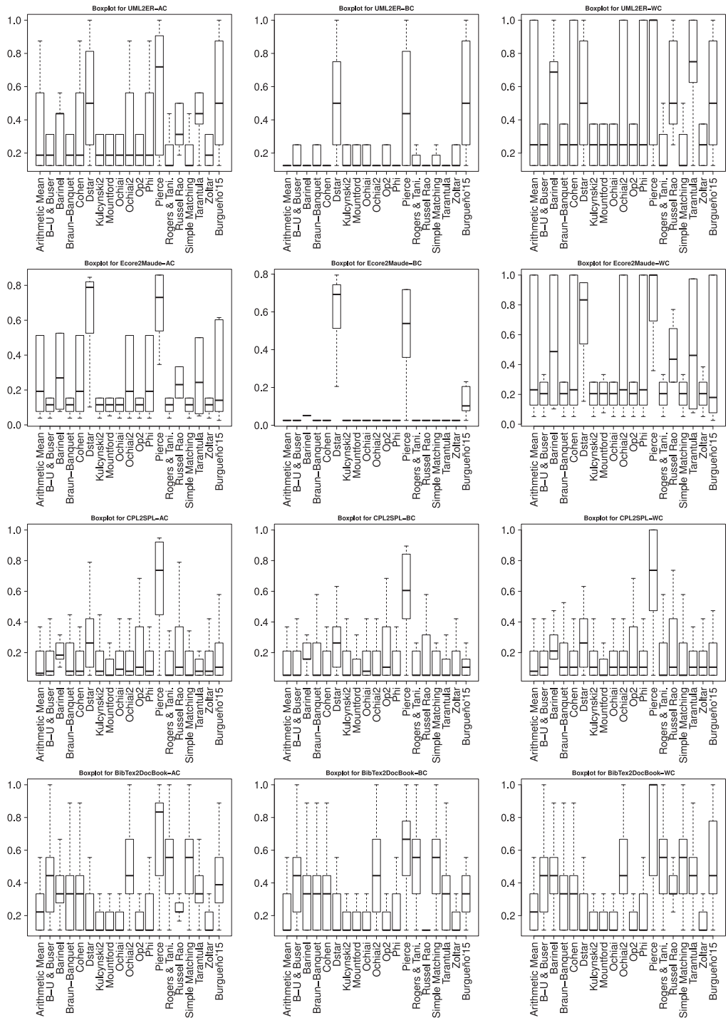
Fig. 8. Box-plot of the EXAM score of each technique per scenario and case study including Reference [18] (Burgueño'15).
