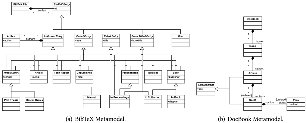
Fig. 2. Metamodels of the BibTeX2DocBook transformation (from Reference [54]).
