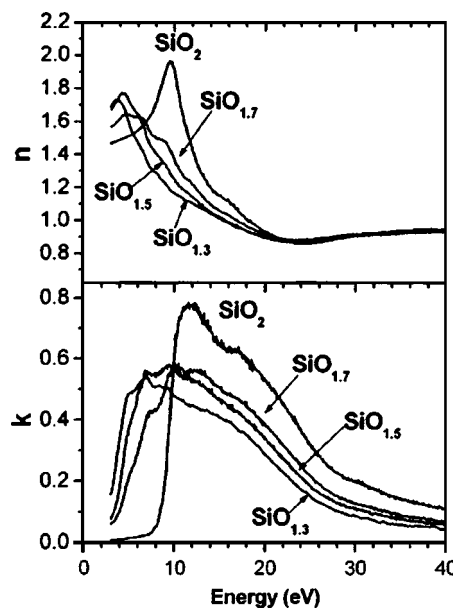
FIG. 10. n and k functions derived from the REELS spectra for the indicated SiO_x samples.
