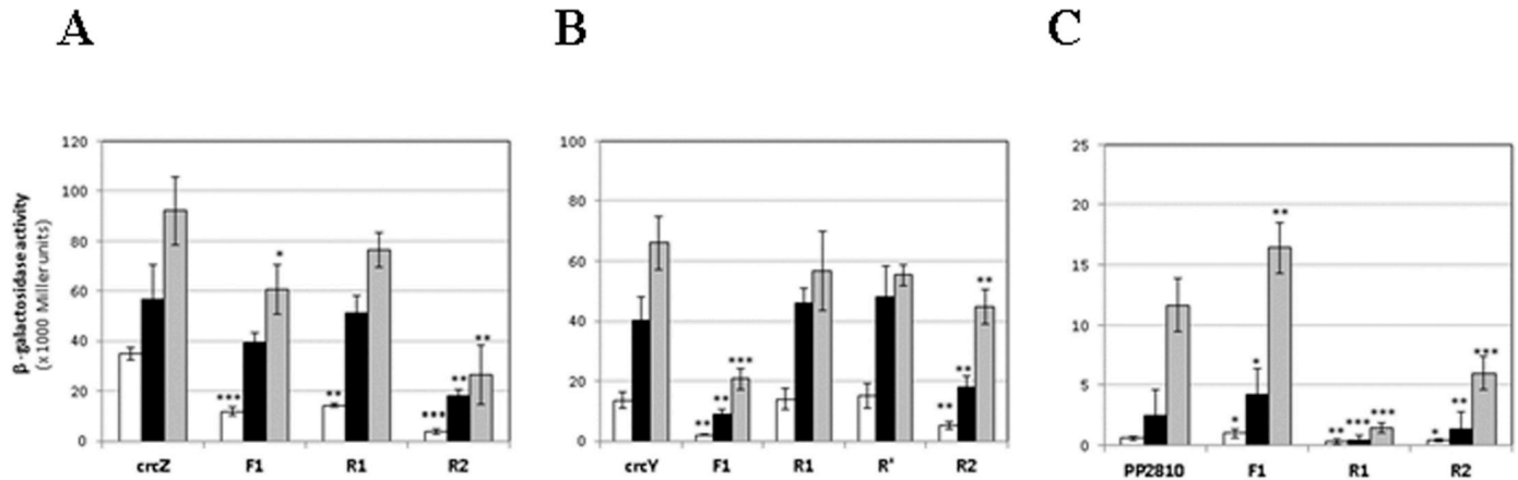
Fig 3. In vivo expression of crcZ , crcY and PP2810 of P. putida and point mutagenesis of the CbrB binding sites. Expression was measured as \beta -galactosidase activity of the crcZ (A), crcY (B) and PP2810 (C) -lacZ transcriptional fusions of the promoter region or the corresponding substituted sites F1, R1 or R2 in LB (white bars), minimal medium with succinate (black bars) and oxaloacetate (grey bars) as carbon source. Plasmids pMPO1316, pMPO1314 and pMPO422 contained the wild type sequences for crcZ , crcY and PP2810 , respectively. Substitutions of F1, R1 (R') and R2 were generated in plasmids pMPO436, pMPO437 and pMPO438 for crcZ , pMPO439, pMPO440 (pMPO441) and pMPO442 for crcY and plasmids pMPO425, pMPO426 and pMPO428 for PP2810 . The values are the average of at least three independent assays. The error bars indicate the standard deviation of the means of at least three independent assays. Stars designate p-values for the Student's t-test for unpaired samples not assuming equal variance and are referred to the wild type sequence of each promoter. *: p<0.05; **: p<0.01; ***: p<0.005.
