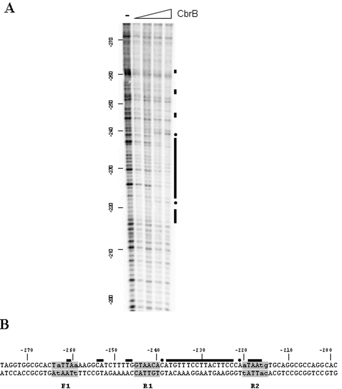
Fig 5. DNase I footprint of CbrB on the PP2810 promoter region. (A) CbrB footprint analysis for a linear fragment containing the promoter region of PP2810 with increasing concentrations of CbrB. CbrB-protected regions to DNase I digestion (black bars), and hypersensitive positions (dots) are marked. The coordinates are relative to the ATG. (B) Schematic representation of the CbrB-protected regions on the sequence of the PP2810 promoter region, with the same references as for the footprint pattern. Shaded boxes on the PP2810 promoter sequence indicate proposed CbrB-binding subsites.
