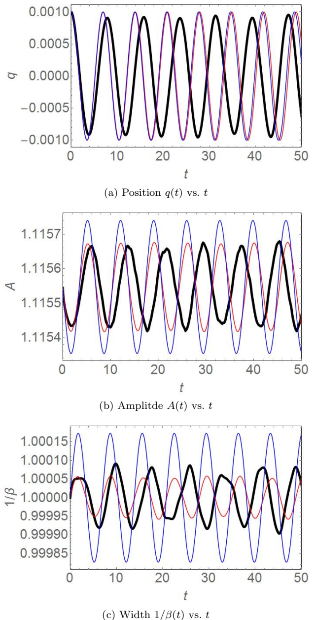
FIG. 4. Comparison of the four CC (blue line), six CC (red line), and numerical simulation (black line) for b = 0.1 . Parameters and initial conditions are m = 1, q_0 = .001 , all other initial conditions are the exact solution values. Here we display q(t) , A(t) , and 1/\beta(t) . For this choice the two linear response periods are: T_q = 7.025 and T_\beta = 4.038 .
