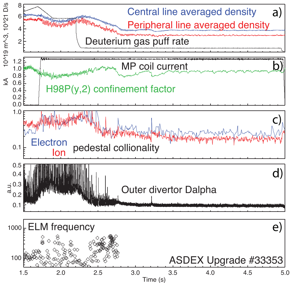
Figure 5. Typical time traces for a low collisionality discharge on AUG where ELM suppression was achieved. Reproduced from [18]. © 2017 Max-Planck-Institut für Plasmaphysik.
