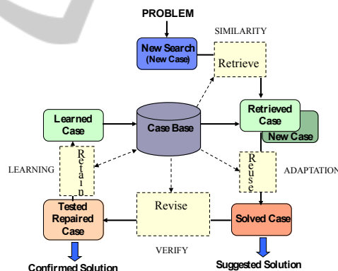
Figure 3: Case Based Reasoning Cycle in OntoUS.
