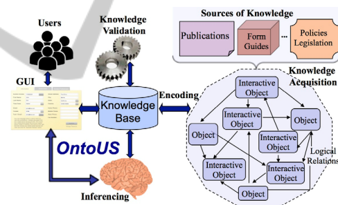
Figure 2: System architecture of OntoUS.
