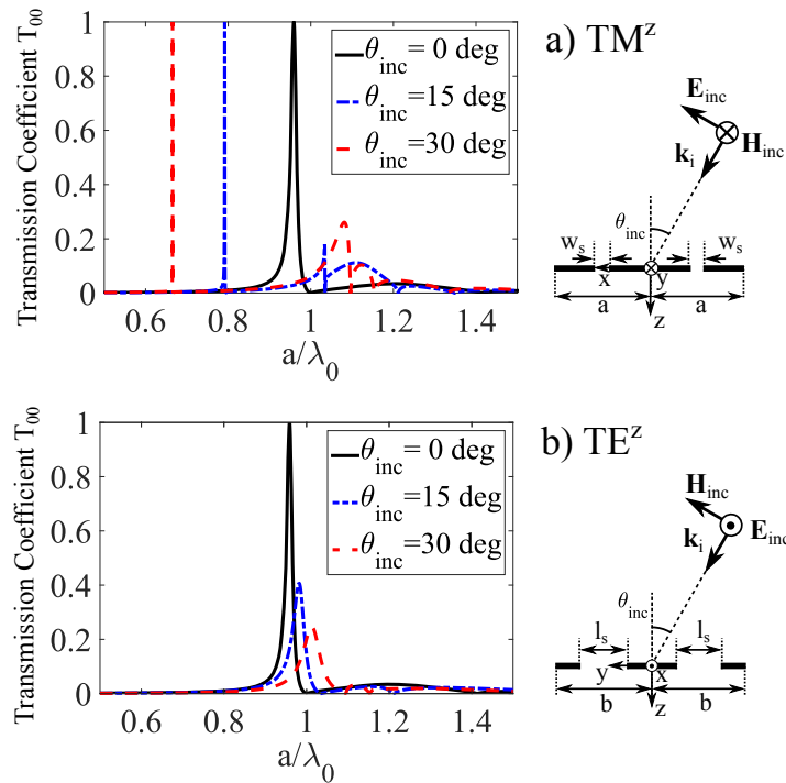
Fig. 3. Transmission spectra of a plane wave impinging on a 2-D array of rectangular slots in a PEC screen. Two polarizations \text{TM}^z (a) and \text{TE}^z (b) are considered, and different angles of incidence ( \theta_{\text{inc}} ). In both cases, the direction of the incident electric field is contained in the x - z plane so as to excite the fields in the slots. The dimensions of the unit cell were chosen to be l_s/a = 0.4 , w_s/a = 0.05 and a = b .
