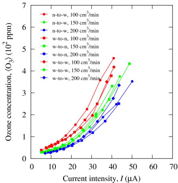
Fig. 7. Ozone concentration as a function of the current intensity (positive corona) for different gas flow rates and flow directions. n-to-w: needle (entry) to lateral port (exit), w-to-n: lateral port (entry) to needle (exit), w-to-w: lateral port (entry) to opposite lateral port (exit).
