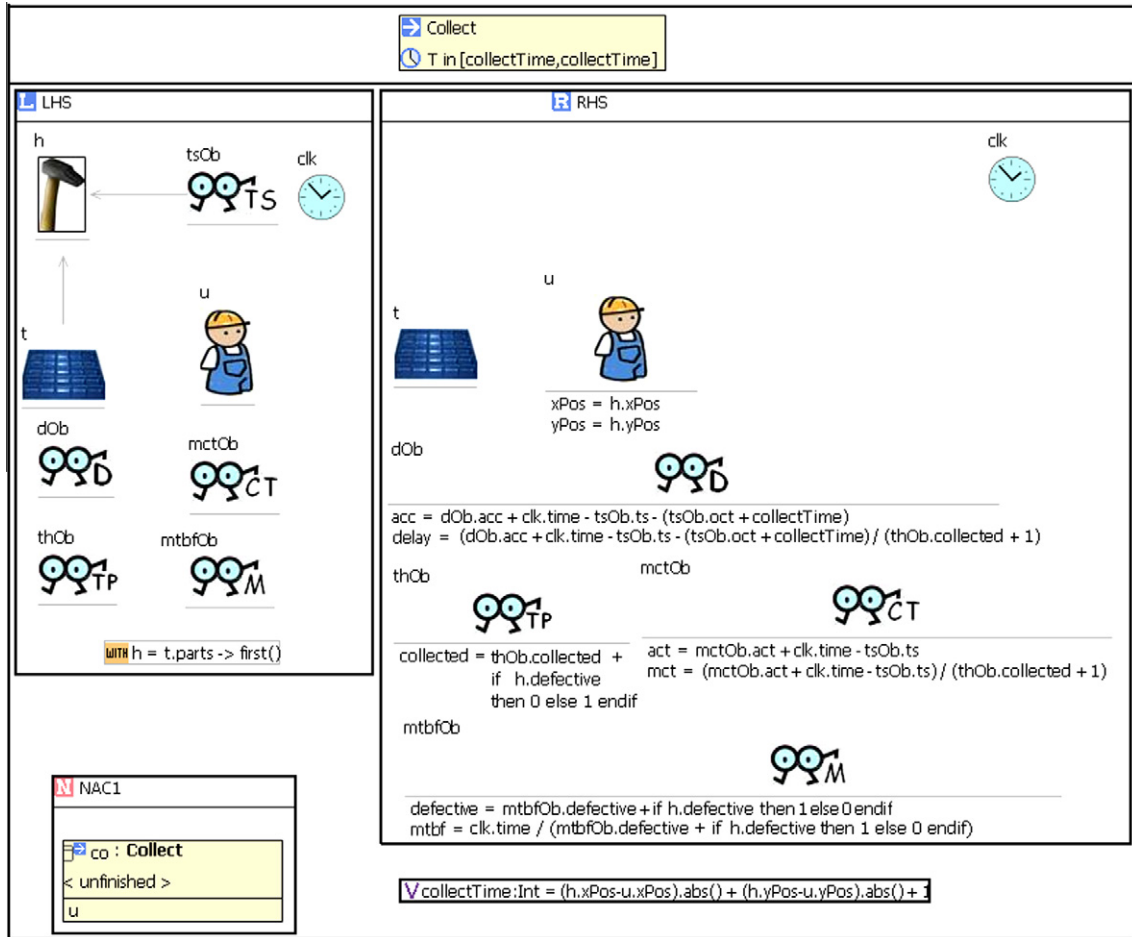
Fig. 10. Collect rule.
