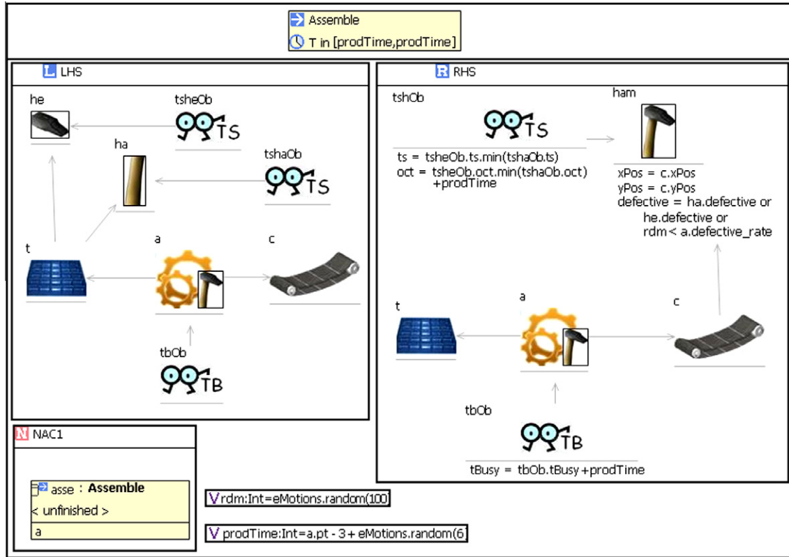
Fig. 9. Assemble rule.
