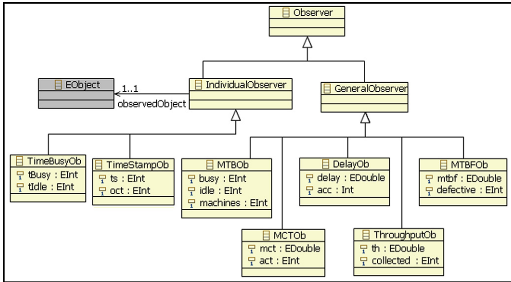
Fig. 4. Observers metamodel.
