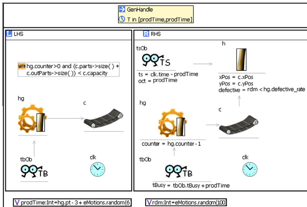
Fig. 6. GenHandle rule.
