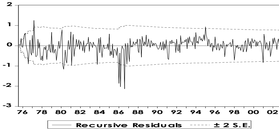
FIGURE 4. RECURSIVE RESIDUALS
