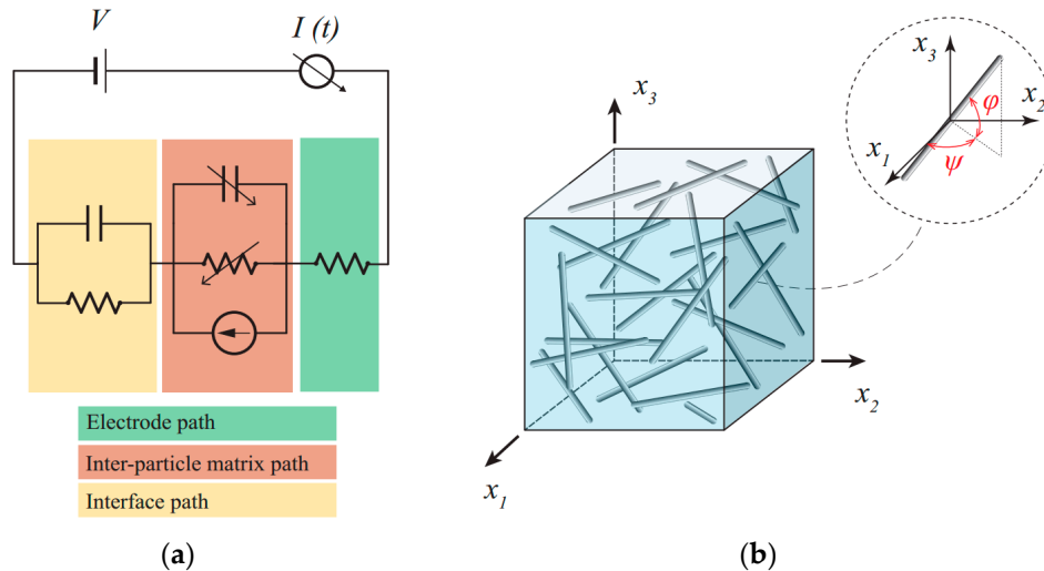
Figure 3. Modeling strategies for self-sensing structural materials: (a) Example of a lumped circuit model; (b) Sketch of a micromechanics modeling approach.
