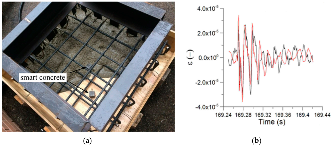
Figure 4. Example application of smart concrete sensors embedded to measure strain in reinforced concrete structures: (a) Photo evidence of the embedded sensor during concrete casting; (b) Comparison of the output of the smart concrete sensor (black line) and of a traditional strain gauge (red line) during a hammer hit test on a RC beam.
