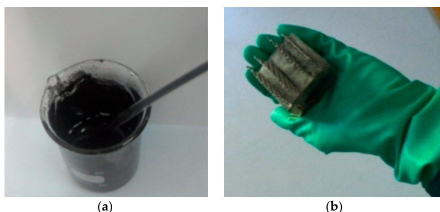
Figure 1. Smart concrete: (a) Dispersion of MWCNT in water for preparation of smart concrete; (b) Cubic sensor made of smart concrete doped with MWCNT.
