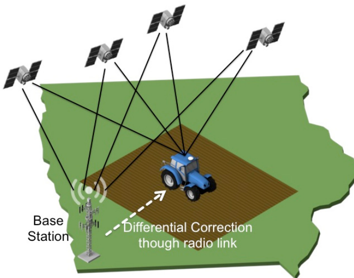
Figure 5. Schematic diagram of a differential correction technique (Courtesy of TRIMBLE)
