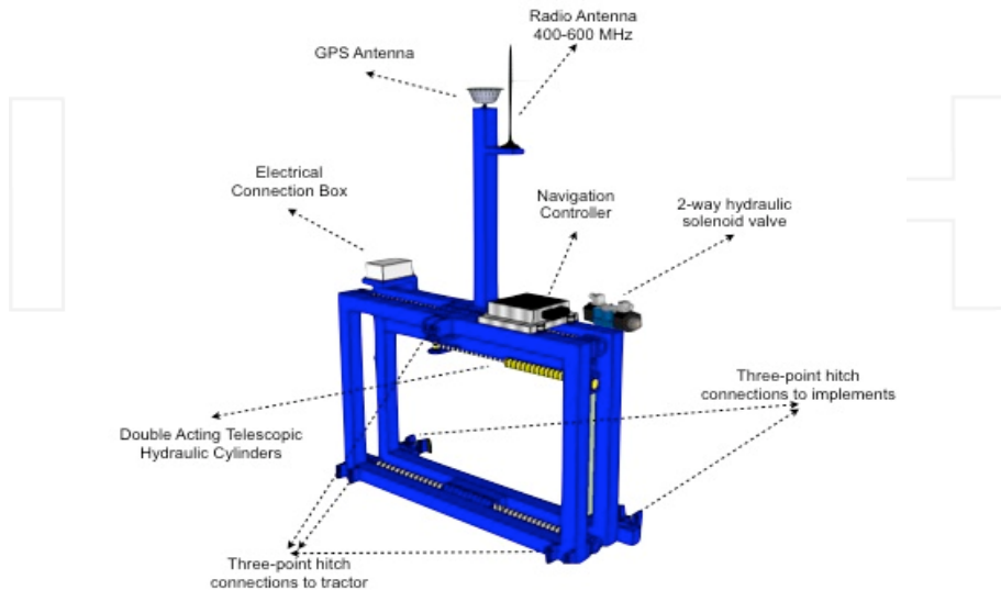
Figure 15. Schematic diagram showing the side-shift frame system developed for row position centering controlled with a RTK-GPS geopositioning system.
