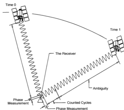
Figure 4. Principle of carrier phase measurement (Source: http://nptel.iitm.ac.in/courses )
