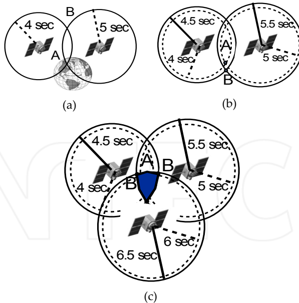
Figure 3. Determination of 2-D position of object A using pseudorangeing principle – (a) no error in time measurement, (b) effect of error in measuring time, and (3) region of uncertainty (or estimate of error) when timing signals from three satellites are utilized for determining position in 2-D.
