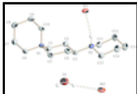
Fig. 1. ORTEP drawing of the asymmetric unit of the title compound, (\text{C}_{15}\text{H}_{30}\text{N}_2)^{2+} \cdot 2(\text{Br}^-) \cdot \text{H}_2\text{O} , with atom labeling and numbering. Atoms are represented by 50% probability thermal ellipsoids except for H atoms, which are shown as small spheres. The dotted line is a hydrogen bond. C-bonded hydrogen atoms have been omitted for clarity.
