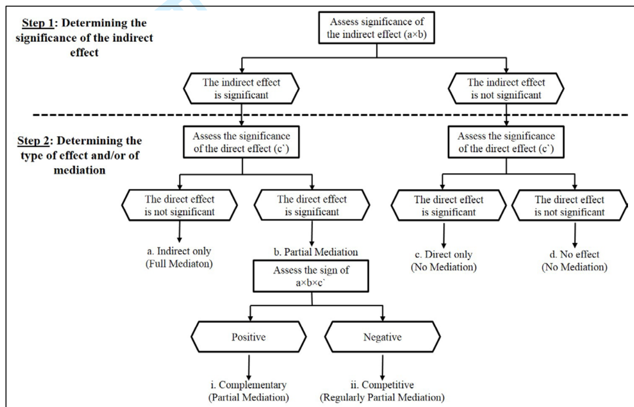
Figure 2: Mediator analysis procedure in PLS (cf. Zhao et al., 2010)
