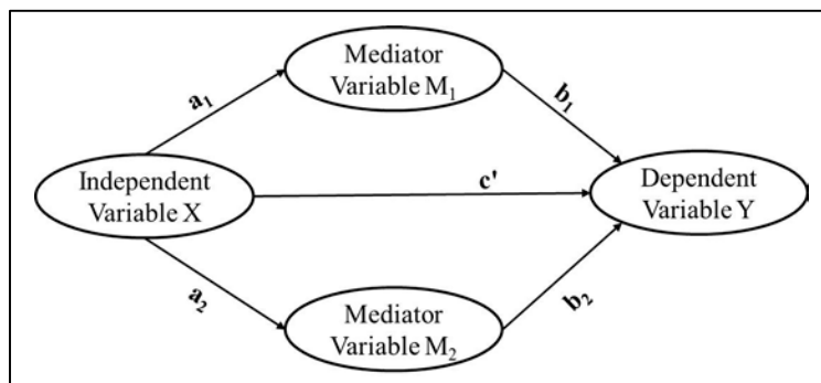
Figure 3: Multiple Mediator Model
