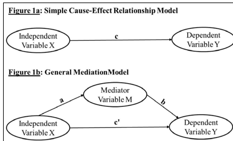
Figure 1: Simple Cause-Effect Relationship and General Mediation Model
