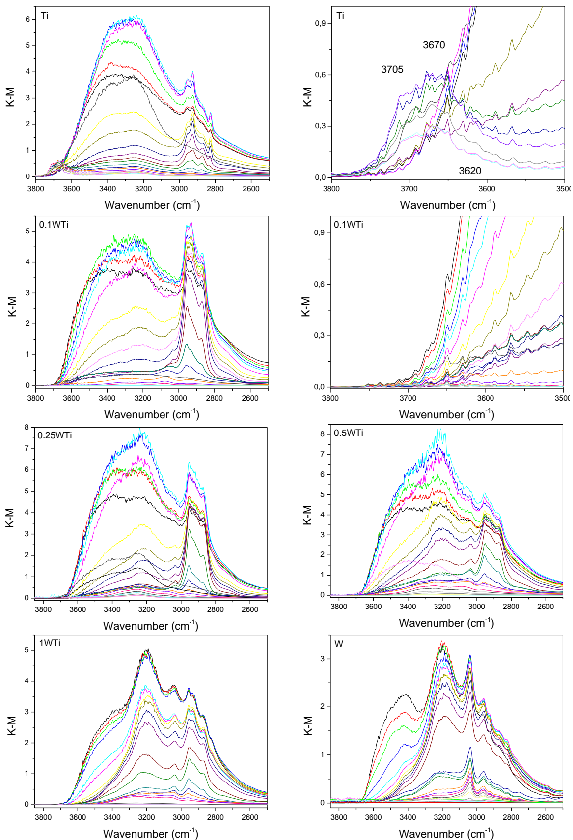
Fig. 9. IR spectra of the Oh region for the WTi and Ti reference samples under a O_2/He temperature ramp. Spectra at RT and each 25 degrees from 50 to 550 °C are presented. Color codes: black RT; red 50 °C; green 75 °C; blue 100 °C; cyan 125 °C; magenta 150 °C; yellow 175 °C; dark yellow 200 °C; navy 225 °C; purple 250 °C; wine 275 °C; Olive 300 °C; dark cyan 325 °C; royal 350 °C; orange 375 °C; violet 400 °C; pink 425 °C; white 450 °C; light gray 475 °C; gray 500 °C; light yellow 525 °C; light cyan 550 °C; dark gray RT. For selected samples an expanded view of the isolated hydroxyl region is presented
