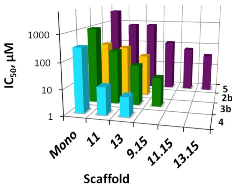
Figure 4. Comparison of the IC_{50} ( \mu\text{M} ) values obtained for similar dendrimers with different monovalent ligands ( 2b , 3b , 4 , 5 )
