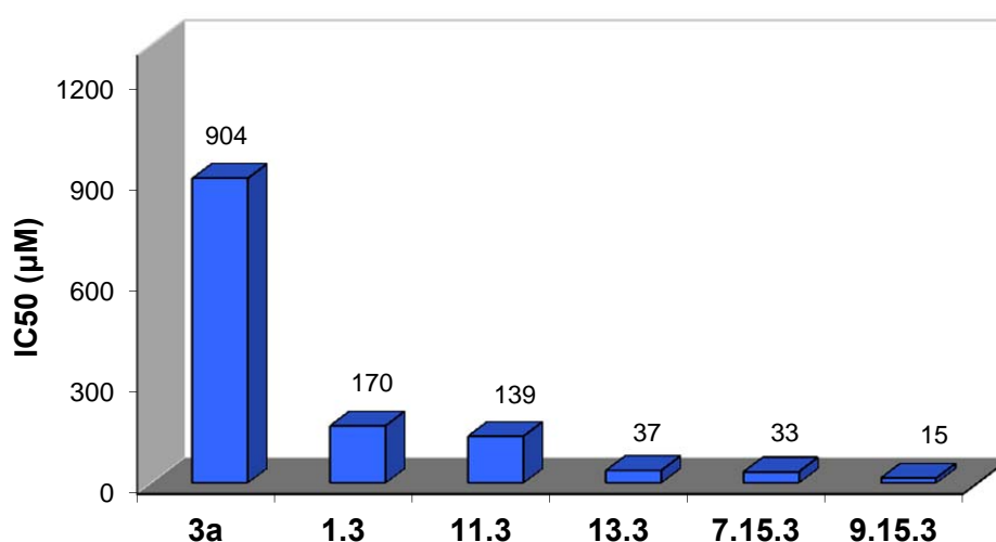
56 57 58 59 60 61 62 63 64 65 Figure 3. Schematic structures and \text{IC}_{50} values of the monovalent pseudo-disaccharide 3a , glycodendron 1.3 (Boltorn type) and glycodendrimers 11.3 , 13.3 , 7.15.3 and 9.15.3 (pentaerythritol based) measured by SPR (competition experiments with immobilized Man-BSA)
