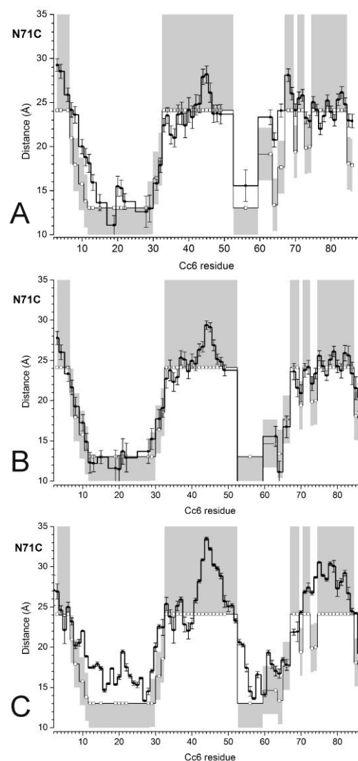
Figure 4. Fitting of the experimental distances. The average distances between the oxygen atom of spin label N71C and Cc6 amide protons were back-calculated from various ensembles (thick line and solid symbols), plotted against the residue number and compared with the experimental distances (open symbols). The grey areas indicate the experimental error margins. In (A, B) the solid line represents the averages for the ten best structures obtained from docking a single copy (A), or ten ensembles of five copies (B) of Cc6. In (C), it represents the averages from three sets of 10,000 randomly selected structures from the MC ensemble. The error bars indicate the SD of the ensembles.
