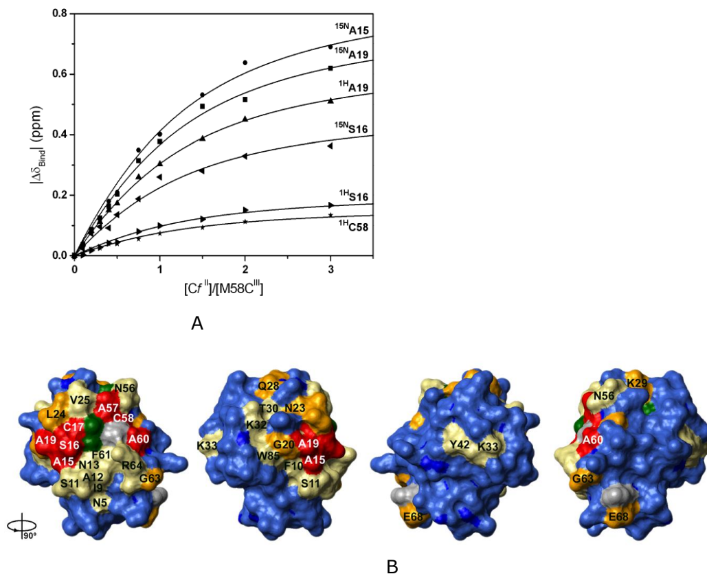
Figure 2. Binding of M58C Cc6 to Cf. A) Binding curves for the interaction of M58C mutant with ferrous Cf. The data were fitted globally to a 1:1 model (non-linear, least-squares), yielding an association constant of 7 (\pm 2) 10^3 \text{ M}^{-1} . B) Chemical shift perturbations map. Residues for which a \Delta\delta_{\text{Avg}} (ppm) was calculated are colour-coded on the structure of M58C mutant according to the following categories: blue for <0.025 ppm, yellow for \geq 0.025 ppm, orange for \geq 0.050 ppm, red for \geq 0.125 ppm. Prolines are shown in grey and the haem group in dark green. Residues are identified with the single-letter amino acid code, and the surfaces have been rotated in anti-clockwise 90^\circ steps around the vertical axis, with respect to the one on the left. Surface representations were generated using MOLMOL.[2]
