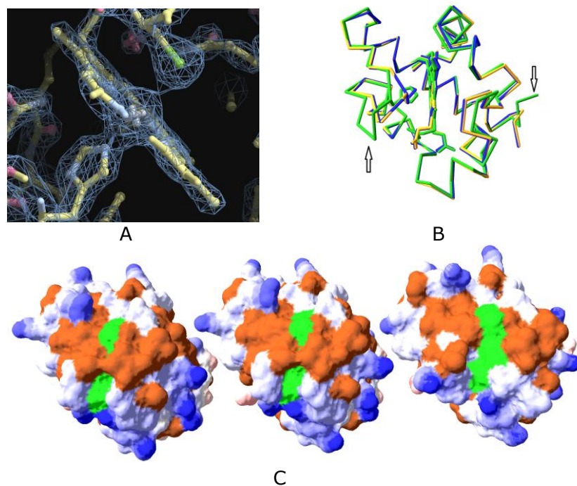
Figure 1. Comparison of Cc6 structures. A) Electron density contoured at 2.2 sigma with the final M58C Cc6 model in the region around the haem iron. This figure was created with COOT.[1] B) Overlay of Ca traces of wt (blue), M58C (yellow) and M58H (green). Residue 58 and the haem are shown in sticks. The arrows indicate the large differences between M58H and wt Cc6. C) Surface representations of M58C (left), wt (middle) and M58H (right). The surface is coloured according to the surface potential from red to blue (negative to positive, calculated with DeepView ( http://www.genebee.msu.su/spdbv )). Non-polar residues are in brown and the haem is in green.
