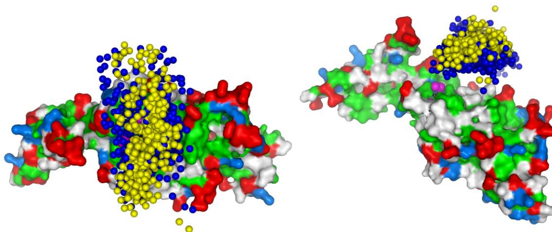
Figure 5. The ensemble of Cc6 around Cf shown in two orientations. Cf is shown in surface representation with the haem in magenta spheres. Negative, positive and hydrophobic residues (including Tyr and Trp) of Cf are displayed in red, marine and green, respectively. The yellow and dark blue spheres represent the centers-of-mass and iron atoms of Cc6 in the ensemble, respectively.
