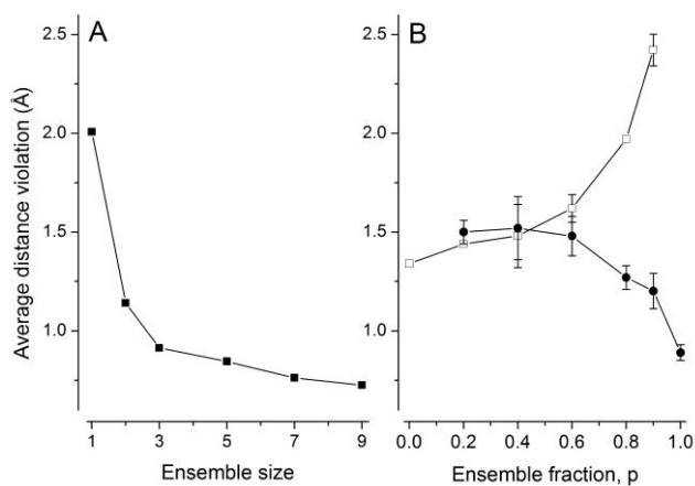
Figure 3. Average violation plots. A) The average distance violation plotted for increasing ensemble size. B) The average distance violation is plotted for different ensemble fractions ( p ). The results for the average violation for the single structure only (open symbols) and for the combination of single structure and ensemble (solid symbols) are shown. For p = 1 , the complex consists entirely of an ensemble. The ensemble size used in these calculations was five. The definition of the error bars is given in the Experimental section.
