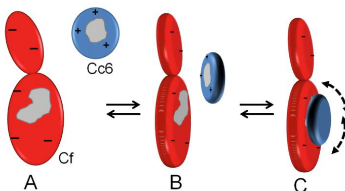
Figure 6. Model for complex formation of Cf and Cc6. A) Free proteins approach via diffusion. B) Electrostatic pre-orientation during approach. C) Cc6 slides over the surface of Cf optimizing hydrophobic contacts (grey areas). Some of the positions in this state are compatible with fast electron transfer.
