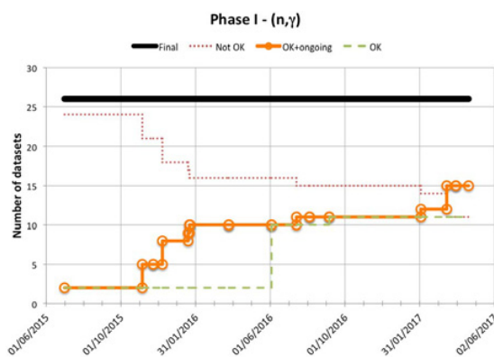
Figure 2. Evolution of data dissemination for (n,\gamma) data (Phase-I). See Fig. 1 for explanation of the legend.
