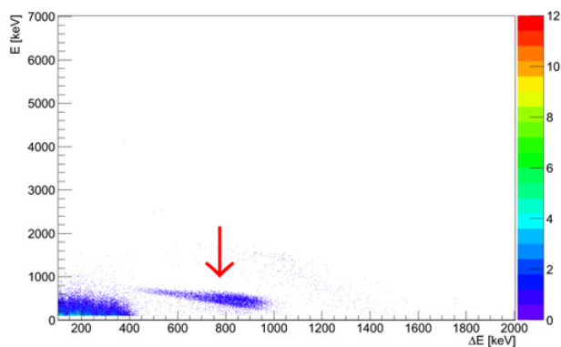
Figure 3. \Delta E -E coincidences matrix for events detected in the telescope. The red arrow points to the region of protons emitted in the {}^7\text{Be}(n,p){}^7\text{Li} reaction.
