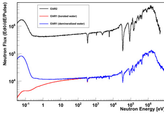
Figure 1. n_TOF neutron flux at EAR1 with normal (blue) and borated (red) water as moderator compared with the neutron flux at EAR2 (black) [8].
