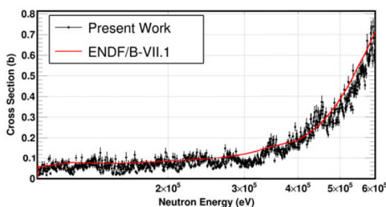
Figure 5. Comparison between present data (black points) and ENDF/B-VII.1 evaluation (red line) in the energy range 100 keV–600 keV. Data is shown using a binning of 2000 bins per energy decade.
