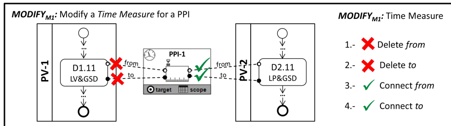
Fig. 1. Example of actions required for an operation MODIFY_M (Time Measure).
