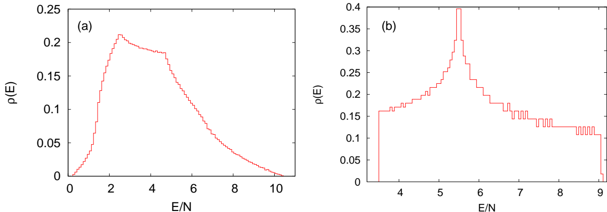
FIG. 7: Density of states \rho(E) : Panel (a) for N = 320 , U = 9 and a molecule at resonance. Panel (b) for N = 2000 without molecule.
