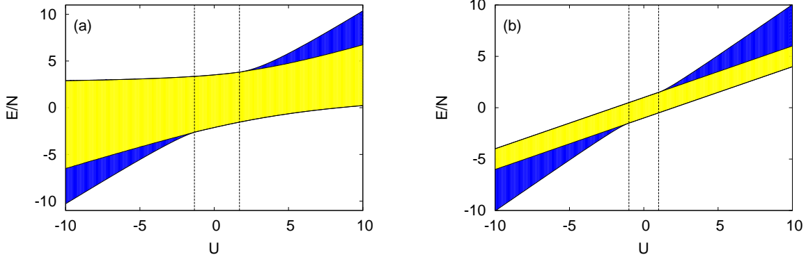
FIG. 6: (Color online) Complete phase diagram. Panel (a) depicts the case with molecule, obtained with N = 320 particles, and J = 1 , \omega = 5 and g = 5 . Panel (b) depicts the case without molecule, with N = 1000 particles and J = 1 . In both cases, dark filled region (blue online) indicates the symmetry-breaking phase, in which the eigenstates are doubly-degenerate, and light filled region (yellow online) the normal phase, in which there are no degeneracies and the parity is a good quantum number for all the eigenstates.
