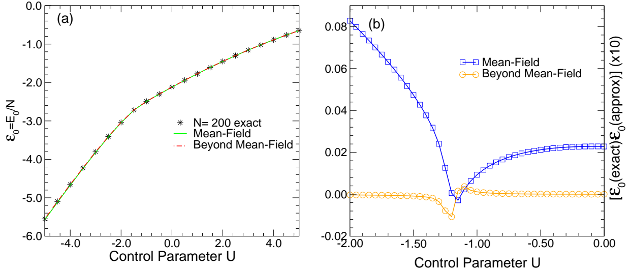
FIG. 4: (Color online) In panel (a) the ground state energy per particle of the model with the diatomic is plotted as a function of the control parameter U for N = 200 . Panel (b) shows the difference between the exact ground state energy per particle obtained numerically and the values obtained by using the two analytic approximations considered in this work in a small region around the critical point for a system with N = 200 . The rest of the control parameters in the Bose-Hubbard Hamiltonian are: J = 1 , \omega = 5 and g = 5 .
