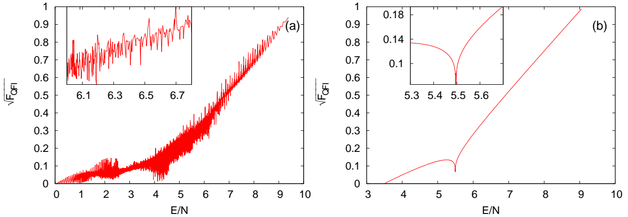
FIG. 9: Fisher information as a function of the energy: Panel (a) for N = 320 , U = 9 and a molecule at resonance. Panel (b) for N = 2000 without molecule.
