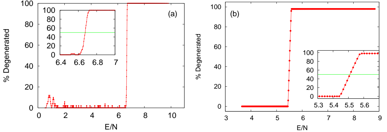
FIG. 8: Ratio of degenerate energy levels as a function of the energy: panel (a) for N = 320 , U = 9 and a molecule at resonance. Panel (b) for N = 2000 without molecule.
