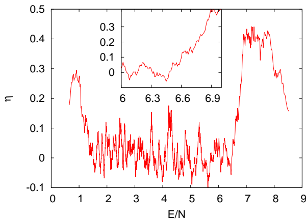
FIG. 10: Spectral statistics for U = 9 and N = 360 , even-parity states, as a function of the scaled energy E/N .
