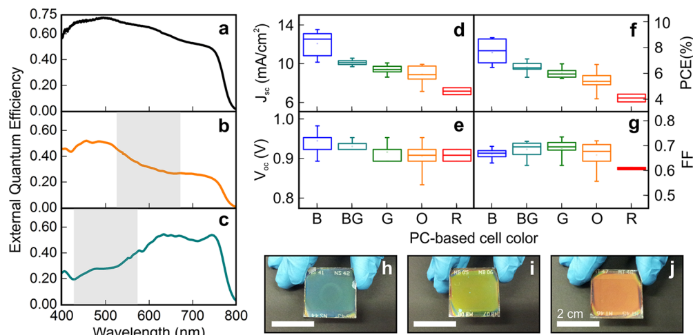
Figure 3. Electrical characterization and device performance analysis. (a–c) Spectral dependence of the external quantum efficiency of (a) a nonphotonic structured \text{SiO}_2 scaffold-based perovskite solar cell, which acts as a reference, (b) an orange PC-based cell, and (c) blue-green PC-based cell. The shaded areas correspond to the spectral regions in which the PC-based cells show high reflectance. (d–g) Box-plot of the device performance indicators for the different PC-based cells: (d) short-circuit current density ( J_{sc} ), (e) open circuit voltage ( V_{oc} ), (f) power conversion efficiency (PCE), and (g) fill factor (FF). (h–j) Digital camera pictures of the devices labeled as (h) blue, (i) green, and (j) orange.
