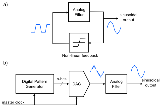
Fig. 1 a) Typical closed-loop sinusoidal signal generator; b) Typical open-loop sinusoidal signal generator
