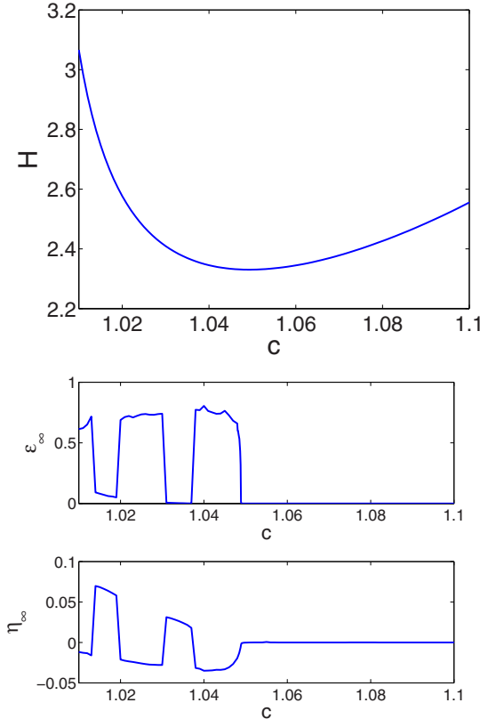
FIG. 3. Stability and instability of the lattice traveling waves of the model of Ref. [14] with the potential in Eq. (10). Here \chi = 4 and u_c = 1 . The top panel displays the H(c) dependence, which possesses a minimum at c = c_0 = 1.0493 . The bottom panels show the dependence of the energy dispersion \varepsilon_\infty and relative velocity change \eta_\infty (see the text) with respect to the velocity c , which manifest the instability of solitary waves with c < c_0 , where c_0 is such that H'(c_0) = 0 .
