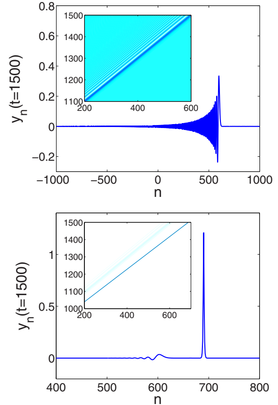
FIG. 4. Evolution of unstable traveling waves in the model of Ref. [14] with the potential in Eq. (10). Here \chi = 4 and u_c = 1 . The panels show the profile of the strains y_n(t) = u_{n+1}(t) - u_n(t) at t = 1500 and zooms in the space-time evolution dynamics of the strains are represented in the insets. Top and bottom panels correspond to c = 1.025 and c = 1.034 , respectively. In the example shown in the bottom panel, the velocity eventually oscillates in time around an average value of 1.0626.
