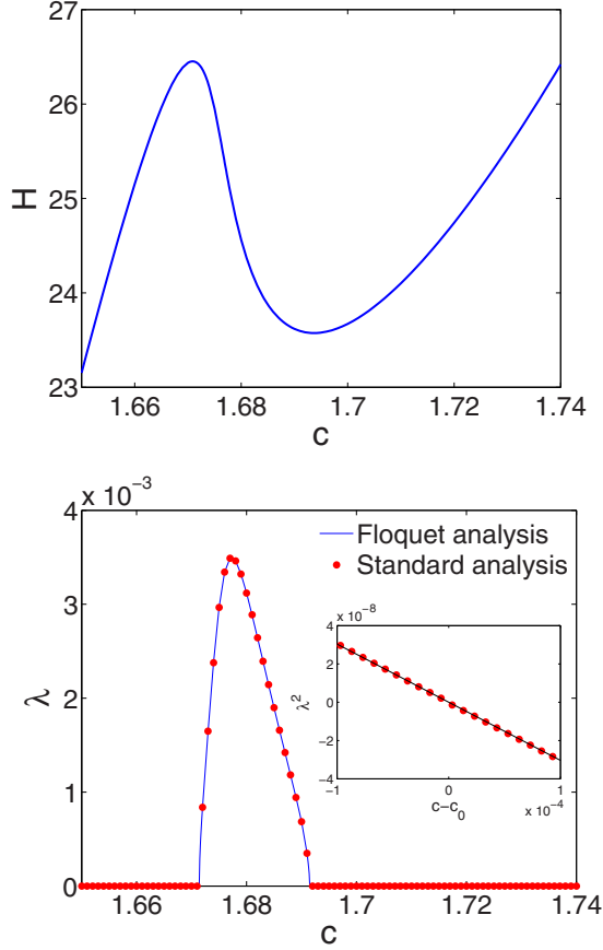
FIG. 2. Stability and instability of the lattice traveling waves in the \alpha -FPU lattice with nearest-neighbor interactions governed by the potential in Eq. (9) and Kac-Baker long-range interactions with the kernel in Eq. (8). Here \gamma = 0.17 and \rho = 0.0172 . The top panel shows the energy dependence on the speed, with H'(c) > 0 implying (spectral) stability, and H'(c) < 0 implying instability. The bottom panel confirms this by showing the maximum real eigenvalue obtained by diagonalizing the linearization operator \mathcal{L} (dots) and transforming the relevant Floquet multiplier \mu into a corresponding eigenvalue (for comparison) via the relation \lambda = c \log(\mu) (solid curve). The inset of the bottom panel shows the dependence of \lambda^2 on c - c_0 for c near c_0 = 1.6937 , the location of the second bifurcation; it fits a straight line \lambda^2 = \beta(c - c_0) , with \beta = -3.0383 \times 10^{-4} .
