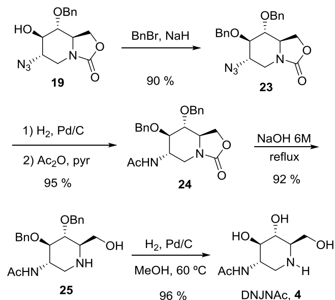
Scheme 4. Synthesis of DNJNac ( 4 ).
