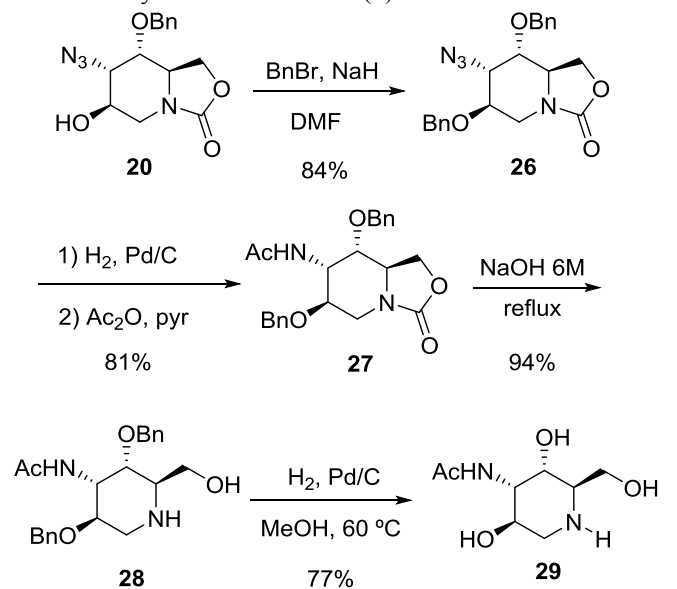
Scheme 5. Synthesis of 3-acetamido-1,3-dideoxyaltronojirimycin ( 29 ).
