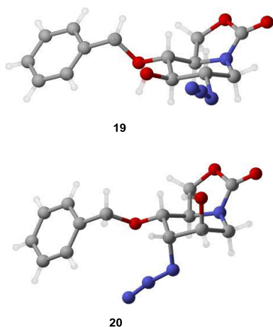
Figure 2. X-ray analysis of azido alcohols 19 and 20 . †
