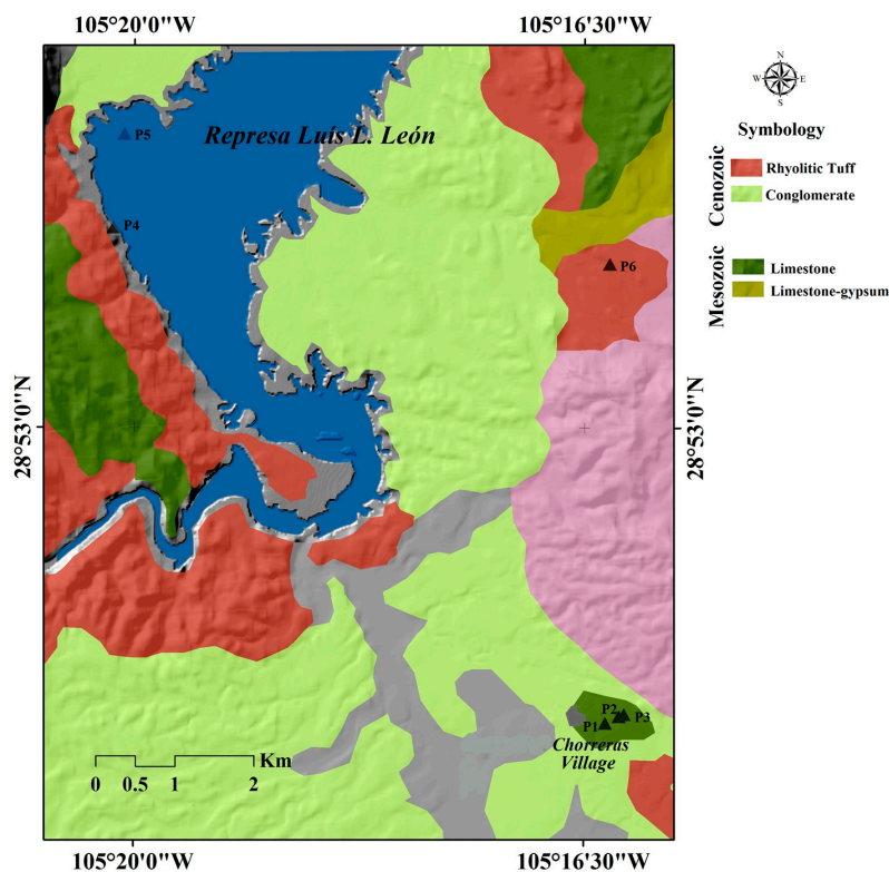
Figure 2. Geological map of Granero reservoir zone.
