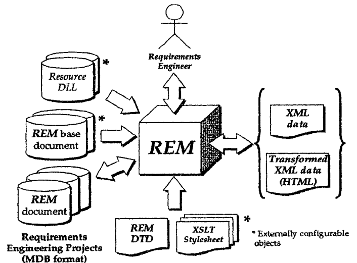
Figure 1: REM Architecture
