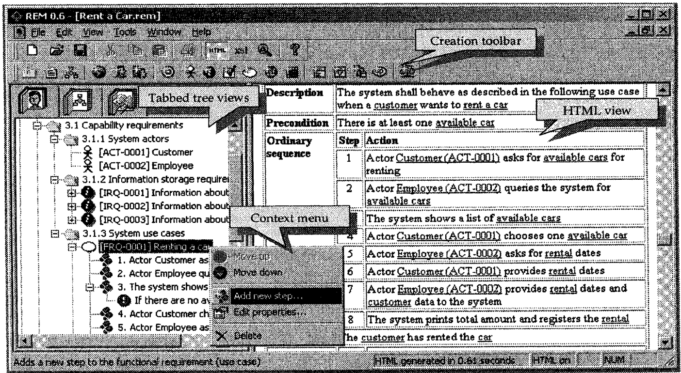
Figure 2: REM User Interface
