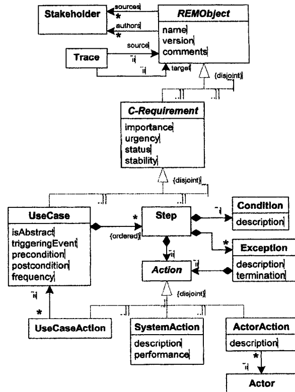
Figure 4: UML model of use cases in REM
