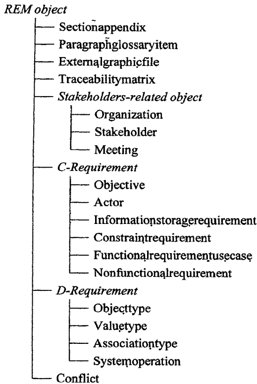
Figure 3: Classification of objects in REM
