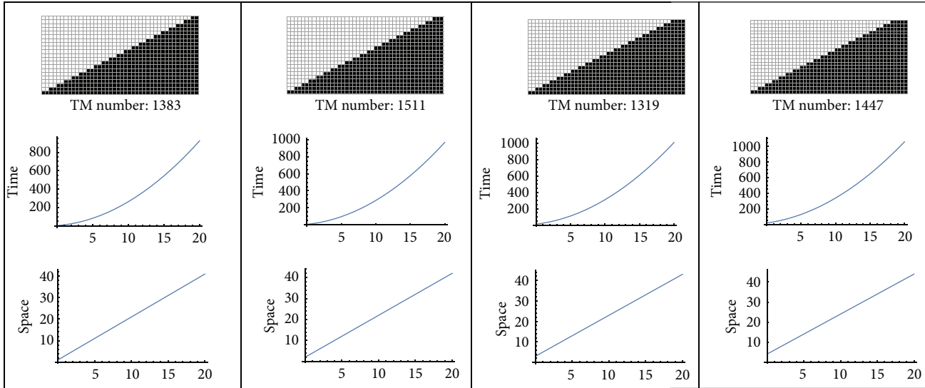
FIGURE 5: The figure shows the four different functions that are computed by the four TMs that have quadratic runtime in (2,2) space. The diagrams show the outputs on increasing inputs. So, for example, in the leftmost diagram, we see that TM with number 1383 (recall this is the code in (2,2) space) outputs two black consecutive cells on input 1, and more in general it outputs 2n black consecutive cells on input n .
