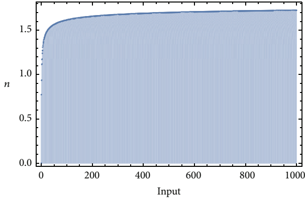
FIGURE 2: The figure shows an estimate of the box dimension of 2,2 TM with TM number 346. On the horizontal axis, the input is shown and the vertical axis shows the corresponding approximation of the box dimension. Note that we know that the function converges to 2 when the input tends to infinity.
