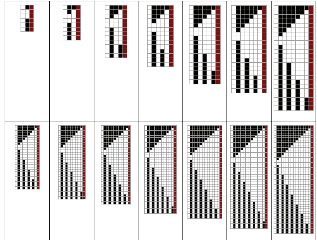
FIGURE 1: The figure shows a sequence of space-time diagrams corresponding to the TM in (2, 2) space with number 346 (according to Wolfram’s enumeration scheme [12, 13] for (2, 2) space) on inputs 1 up to 14.
