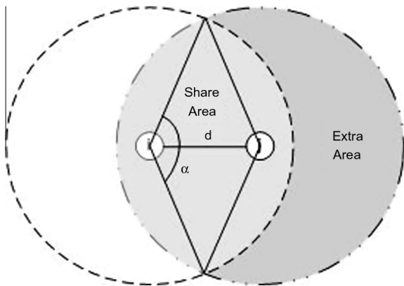
Fig. 9. Share and extra area of two nodes.
