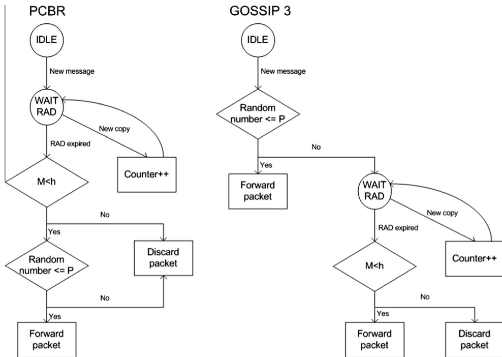
Fig. 13. Difference between GOSSIP3 and PCBR.
