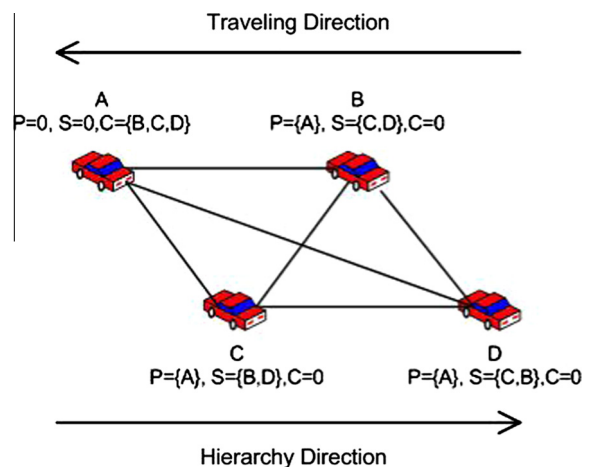
Fig. 4. Node's relationships in PbG.
