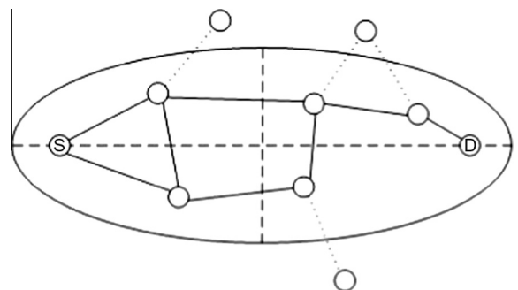
Fig. 10. Forwarding area in regional GOSSIP.
