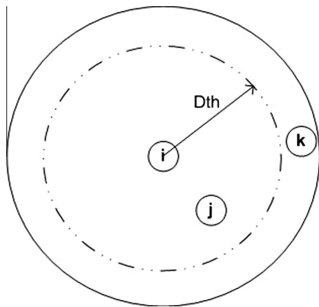
Fig. 14. Distance threshold in Discount scheme.
