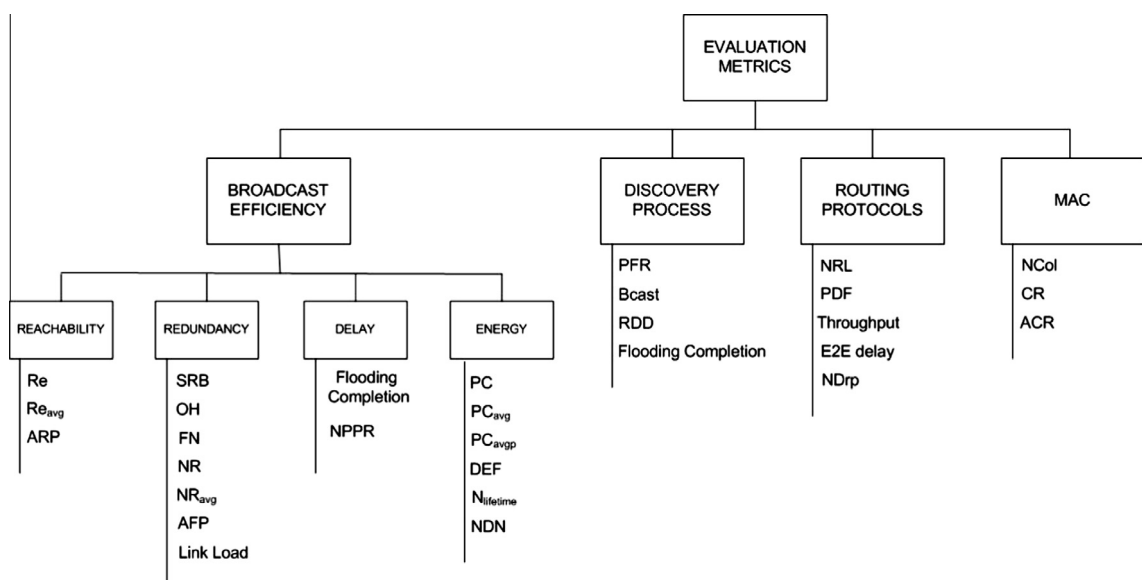
Fig. 15. Classification of the evaluation metrics.
