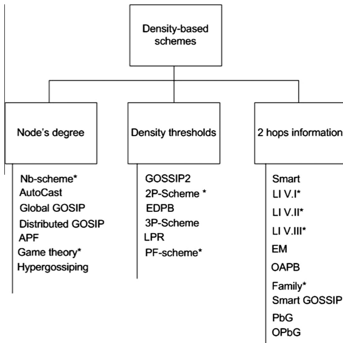
Fig. 3. Classification of density-based schemes.
