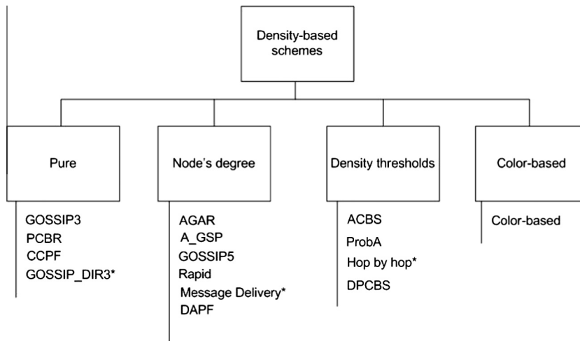
Fig. 11. Classification of density-based schemes.
