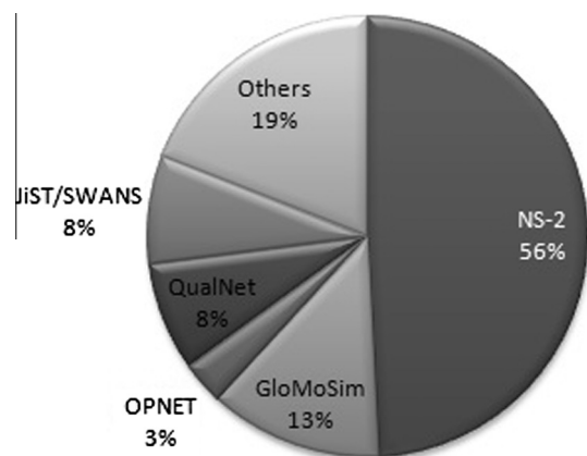
Fig. 18. Network simulators.
