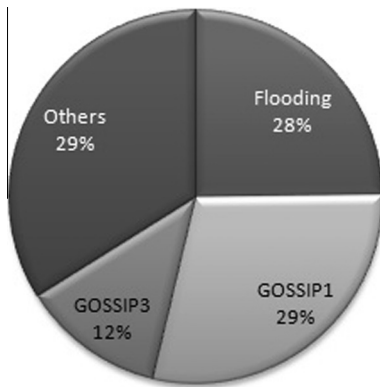
Fig. 16. Comparison schemes.
