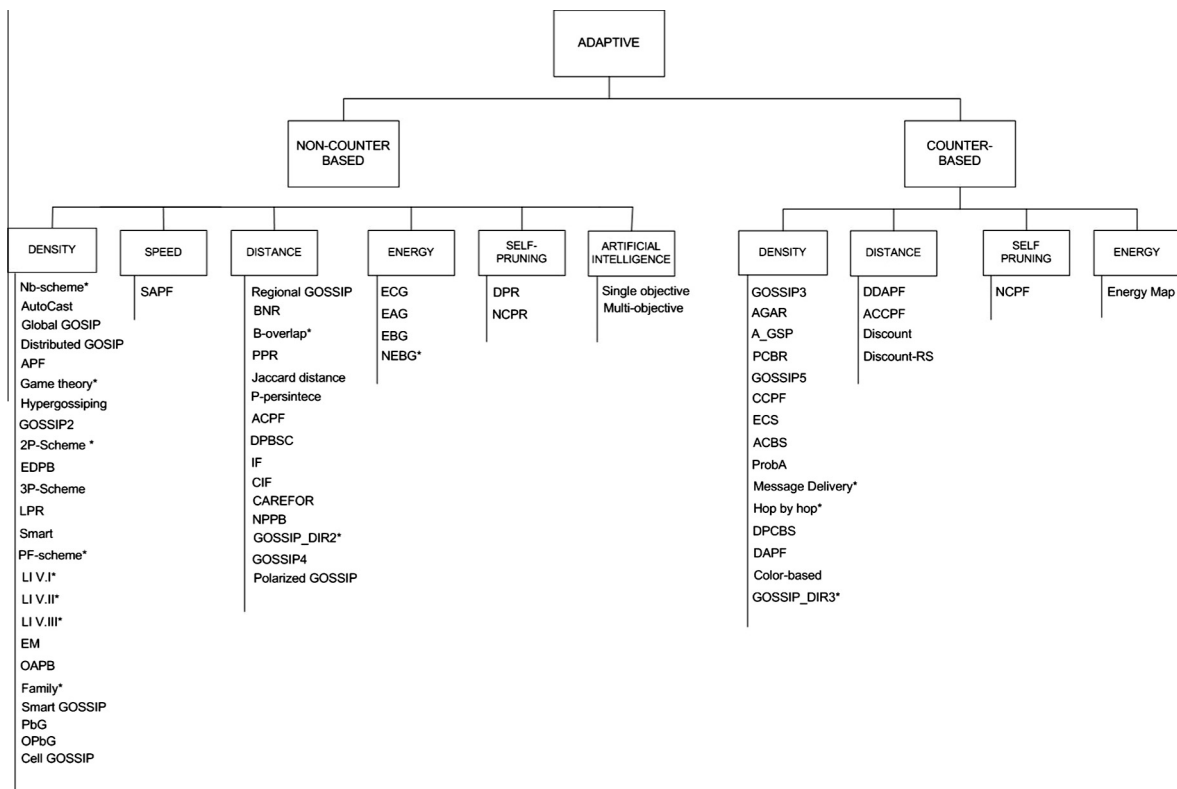
Fig. 2. Classification of adaptive schemes.
