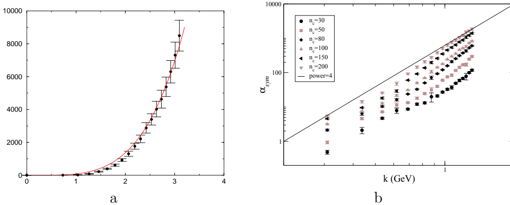
Figure 2: (a) Coupling constant in a cooled lattice ( L = 24, \beta = 6.0 ) after 200 cooling sweeps. The solid line corresponds to the fit discussed in the text. The horizontal axis is given in GeV, assuming for simplicity the lattice spacing of the thermalised configurations, a^{-1} = 1.97 GeV. (b) Coupling constant in a cooled lattice ( L = 24, \beta = 5.6 ) after several cooling sweeps. The horizontal axis is the momentum assuming the same lattice spacing, a^{-1} = 0.83 GeV, which is the value for the thermalised configurations. This is a log-log plot which exhibits better the power law. There seems to be three regimes.
