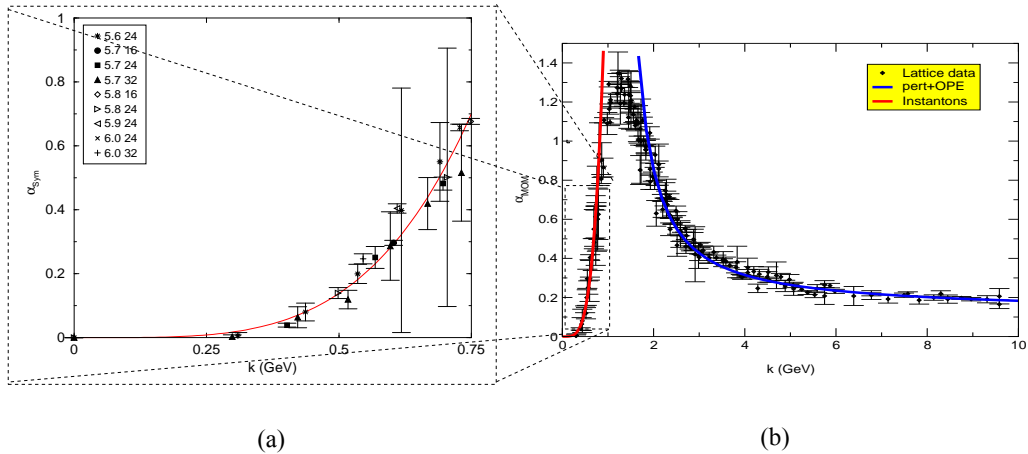
Figure 1: (b) Symmetric MOM coupling constant for different lattice settings and fits to perturbative expression plus power corrections in the high momenta region and to expression (14) discussed in the text for small momenta. (a) Region of small momenta is zoomed.
