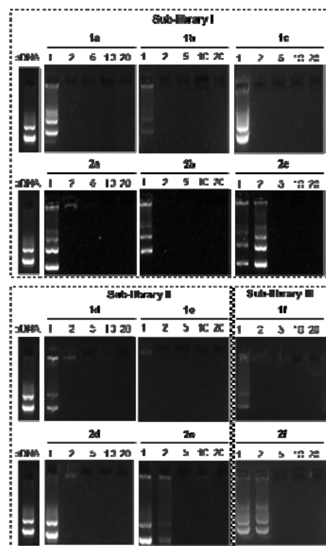
Figure 4. Electrophoresis mobility shift assays (EMSA) for pDNA complexes formulated with 1a-f and 2a-f at different N/P ratios (1, 2, 5, 10 and 20). GelRed TM was used as staining reagent. Naked pDNA was used as negative control.
