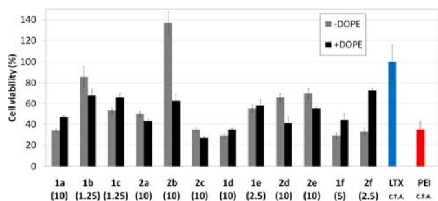
Figure 10. Cell viability of COS-7 cells (MTT determination) in the presence of nanocomplexes formulated with the pEGFP-C1 and \beta CD or CA 4 polycations 1a-f or 2a-f at their optimal concentration ( \mu M) with and without DOPE (1:2 vector-DOPE molar ratio). Data for lipoplexes formulated with Lipofectamine® (LTX), and polyplexes formulated with polyethyleneimine (PEI) are also shown. C.T.A.: Commercial Transfection Agent.
