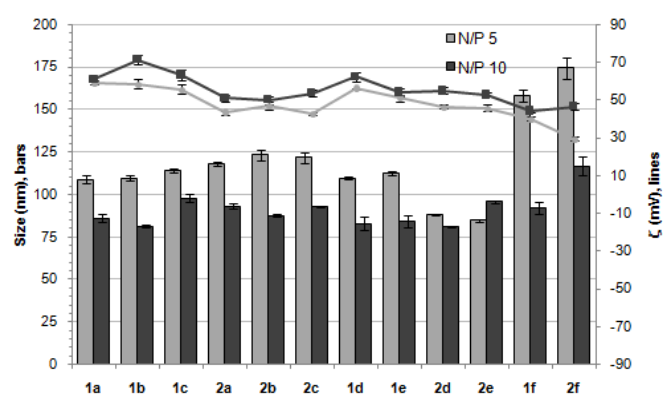
Figure 5. Hydrodynamic diameter (bars, nm) and \zeta potential (lines, mV) of complexes pDNA–polycationic amphiphilic derivatives determined by DLS and M3-PALS analysis.
