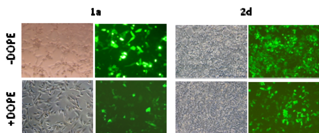
Figure 14. Optical (left columns) and fluorescent (right columns) microscopy images of human RD-4 cells transfected (in green) upon treatment with EGFP-C1 pDNA (1 nM) formulated with polyaminothiourea \beta CD derivative 1a and polyarginine CA 4 derivative 2d .
