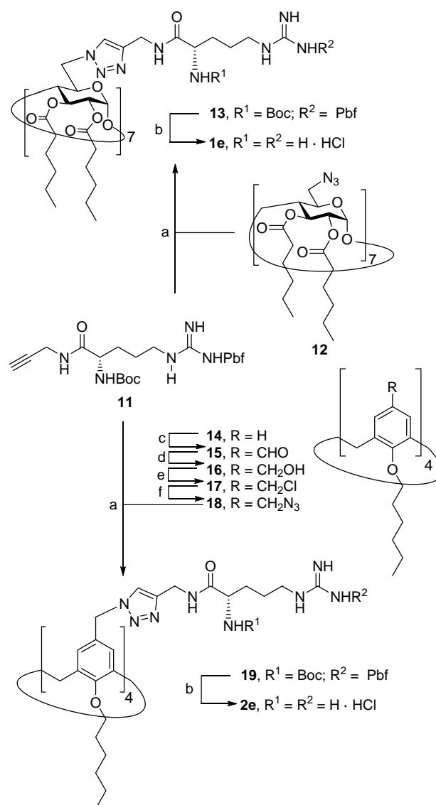
Scheme 3. Synthesis of triazol-linked polyarginine \beta CD and \text{CA}_4 “clicked” clusters 1e and 2e . Reagents and conditions: a) \text{CuI} \cdot \text{P}(\text{OEt})_3 , DIPEA, acetone, reflux, 48 h, 99% (for 13 ) or 24 h, 71% (for 19 ); b) i, 95:2.5:2.5 TFA-TIS- \text{H}_2\text{O} , rt, 1 h; ii, 0.1 M HCl, quantitative; c) i, hexamethylenetetramine, TFA, reflux, 2 d; ii, HCl, 3 h, 96%; d) \text{NaBH}_4 , EtOH, 0^\circ\text{C} \rightarrow \text{rt} , 18 h, 86%; e) \text{SOCl}_2 , DCM, 4 h, rt, 95%; f) \text{NaN}_3 , DMF, 16 h, 40^\circ\text{C} , 95%.
