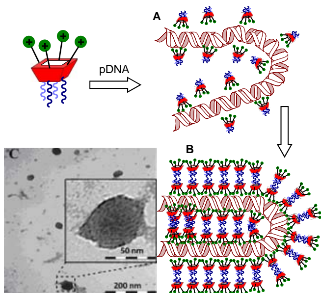
Figure 6. Schematic representation of the proposed mechanism for pDNA complexation by polycationic amphiphilic macrocycles (the general cartoon for CA 4 derivatives in Figure 1 has been used) involving electrostatically-driven templating (A) and bilayer zipping/nanocondensation (B). The TEM micrograph corresponding to the nanocomplexes formulated with compound 1d at N/P 10, is also presented (C). The typical snake-like ultra-thin structure can be appreciated in the insert.
