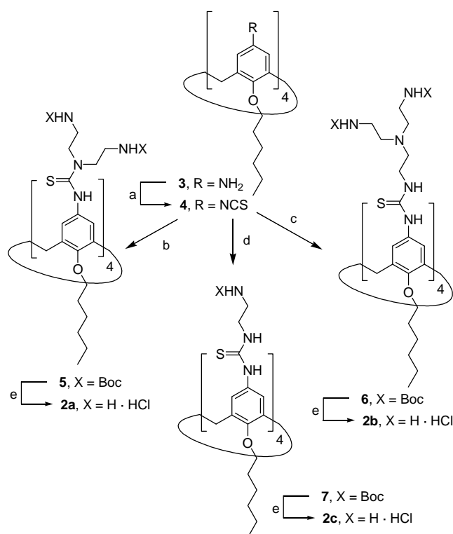
Scheme 1. Synthesis of polyaminothioureido CA 4 derivatives 2a-c . Reagents and conditions: a) i, CS 2 , Et 3 N, EtOH, rt, 2 h; ii, Boc 2 O, DMAP, EtOH, 0 °C \rightarrow rt, 2 h, 88 %; b) NH(CH 2 CH 2 NHBoc) 2 , Et 3 N, DCM, rt, 12 h, quantitative; c) H 2 NCH 2 CH 2 N(CH 2 CH 2 NHBoc) 2 , Et 3 N, DCM, rt, 12 h, 99%. d) NH 2 CH 2 CH 2 NHBoc, Et 3 N, DCM, rt, 1.2 h, 99%; e) i, TFA/TES/DCM, 5 min, rt; ii, HCl, 99%.
