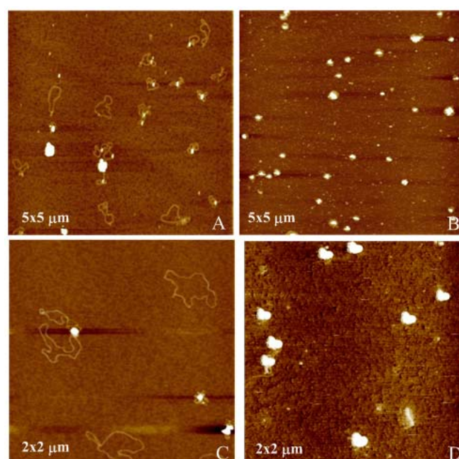
Figure 7. AFM images recorded in tapping mode on air showing the effects induced on EGFP-C1 plasmid DNA folding by incubation with polyguanidino \beta CD and CA 4 derivatives 1f and 2f at N/P 0.5 (A and C) or N/P 5 (B and D).
