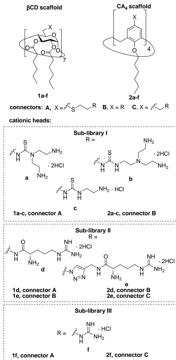
Figure 3. Structures of the polycationic amphiphilic \beta CD and CA 4 derivatives synthesized and evaluated in this work.
