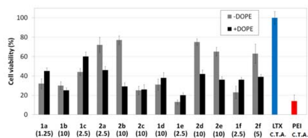
Figure 12. Cell viability of RD-4 cells (MTT determination) in the presence of nanocomplexes formulated with the pEGFP-C1 and \beta CD or CA 4 polycations 1a-f or 2a-f at their optimal concentration ( \mu M) with and without DOPE (1:2 vector-DOPE molar ratio). Data for lipoplexes formulated with Lipofectamine® (LTX), and polyplexes formulated with polyethyleneimine (PEI) are also shown. C.T.A.: Commercial Transfection Agent.
