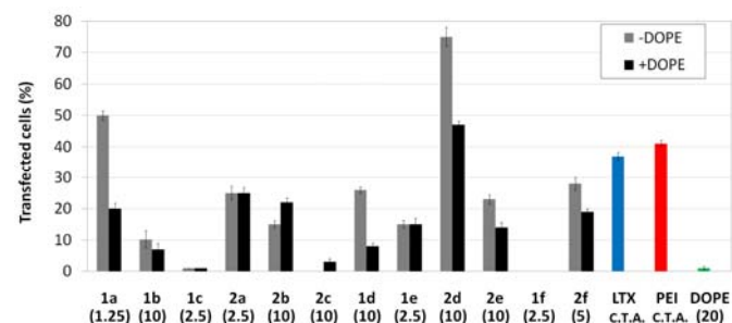
Figure 13. In vitro transfection efficiency in RD-4 cells in the presence of nanocomplexes formulated with the pEGFP-C1 and \beta CD or CA 4 polycations 1a-f or 2a-f at their optimal concentration ( \mu M) with and without DOPE (1:2 vector-DOPE molar ratio). Data for lipoplexes formulated with Lipofectamine® (LTX), and polyplexes formulated with polyethyleneimine (PEI) are also shown. C.T.A.: Commercial Transfection Agent.
