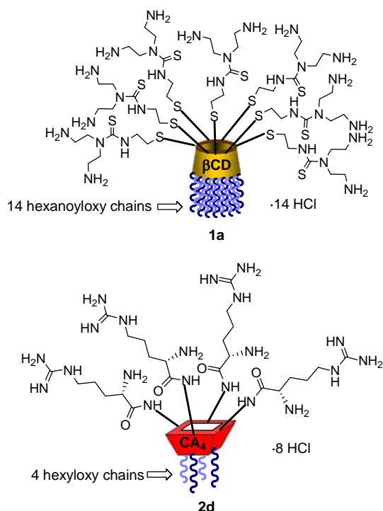
Figure 2. Schematic representation of the lead \beta CD and CA_4 vectors 1a and 2d .
