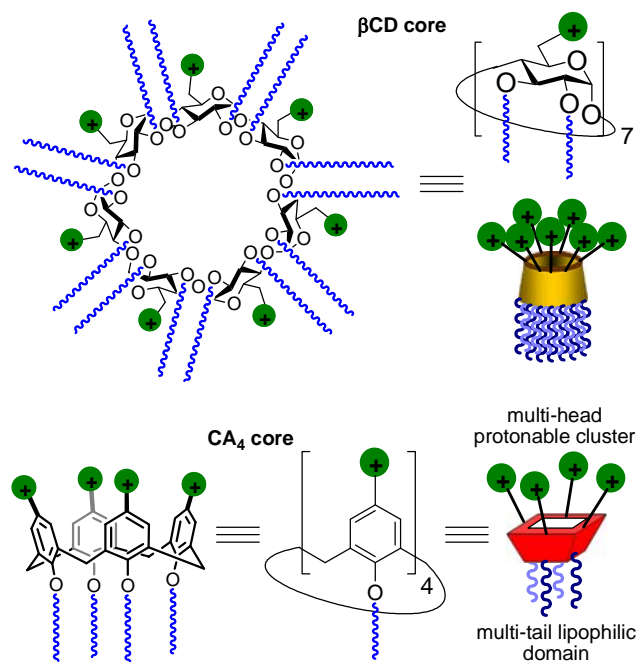
Figure 1. Schematic representation of the amphiphilic polycationic \beta -cyclodextrin ( \beta CD) and calix[4]arene ( CA_4 ) gene vector prototypes in the optimal skirt-type and upper-rim protonable cone arrangements, respectively.
