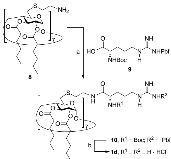
Scheme 2. Synthesis of amide-linked polyarginine \beta CD derivative 1d . Reagents and conditions: a) HBTU, DIPEA, DCM, rt, 12 h, 68%; b) i, 95:2.5:2.5 TFA-TIS-DCM, rt, 1 h; ii, 0.1 M HCl, quantitative. Pbf: 2,2,4,6,7-pentamethyl-dihydrobenzofuran-5-sulfonyl. HBTU: o-(Benzotriazol-1-yl)-N,N,N',N'-tetramethyluronium hexafluorophosphate. DIPEA: Diisopropyl ethyl amine. TIS: triisopropylsilane
