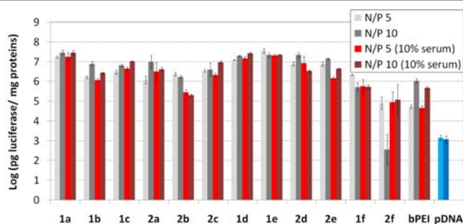
Figure 8. In vitro transfection efficiency in COS-7 cells for CDplexes and calixplexes formulated with 1a-f and 2a-f and pTG11236 plasmid at N/P 5 and 10, in the absence or in the presence of serum (10%). Polyplexes formulated with brached PEI (bPEI) and naked pDNA in the absence (light blue) and presence (dark blue) of 10% serum were included as positive and negative controls, respectively.
