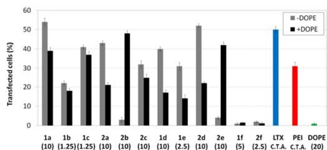
Figure 11. In vitro transfection efficiency in COS-7 cells in the presence of nanocomplexes formulated with the pEGFP-C1 and \beta CD or CA 4 polycations 1a-f or 2a-f at their optimal concentration ( \mu M) with and without DOPE (1:2 vector-DOPE molar ratio). Data for lipoplexes formulated with Lipofectamine® (LTX), and polyplexes formulated with polyethyleneimine (PEI) are also shown. C.T.A.: Commercial Transfection Agent.
