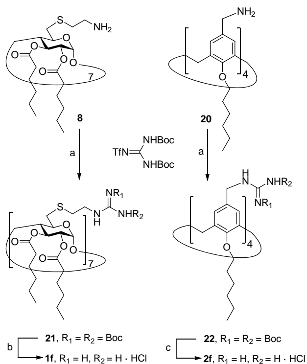
Scheme 4. Synthesis of polyguanidino \beta CD and \text{CA}_4 derivatives 1f and 2f . Reagents and conditions: a) \text{Et}_3\text{N} , DCM, rt, 12 h, 99% (for 21 ) or 48 h, 91% (for 22 ); b) i, 1:1 TFA-DCM, rt, 3 h; ii, 0.1 M HCl, 99%; c) TES, dioxane, 0.1 M HCl, rt, 24 h, quantitative
