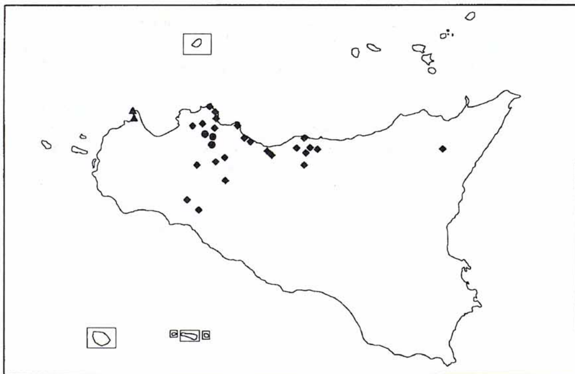
Fig. 3. Distribution of Brassica rupestris : (◆) subsp. rupestris , (●) subsp. hispida , (▲) subsp. brevisiliqua .
