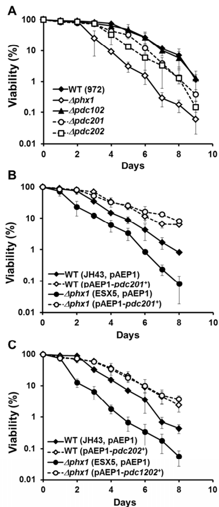
Figure 3. Pdc201 and Pdc202 contribute to long-term survival. (A) Long-term survival of the wild type (WT; 972), \Delta phx1 (JY01 in 972 background), \Delta pdc102 , \Delta pdc201 , and \Delta pdc202 mutants. Viability assay was done as described in the text. At least three independent experiments were carried out to obtain survival curves for each strain. (B) Effect of overproducing Pdc201. Viability of wild type (JH43) and \Delta phx1 mutant (ESX5 in JH43 background) cells with pAEP1- pdc201 + plasmid or parental plasmid were measured as in (A). (C) Effect of overproducing Pdc202. Viability of wild type (JH43) and \Delta phx1 (ESX5) cells containing pAEP1- pdc202 + plasmid or parental plasmid were measured.
