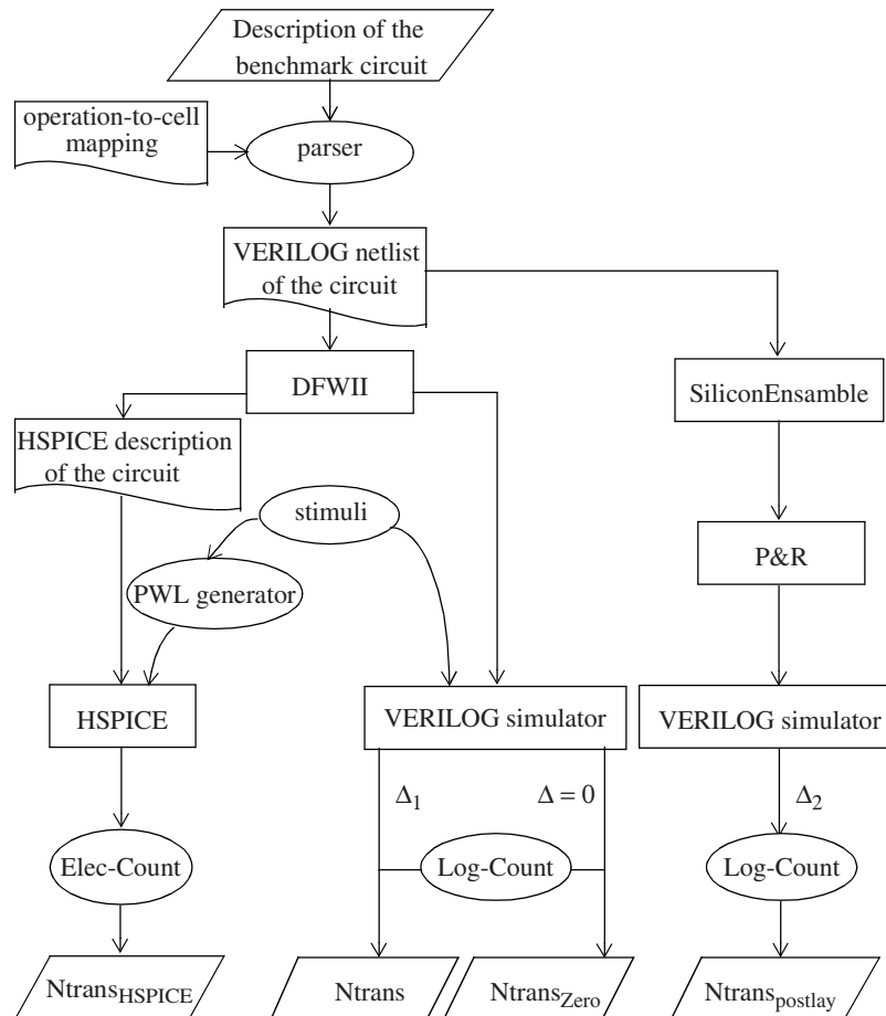
Figure 1 . A scheme of the method for switching activity computation
