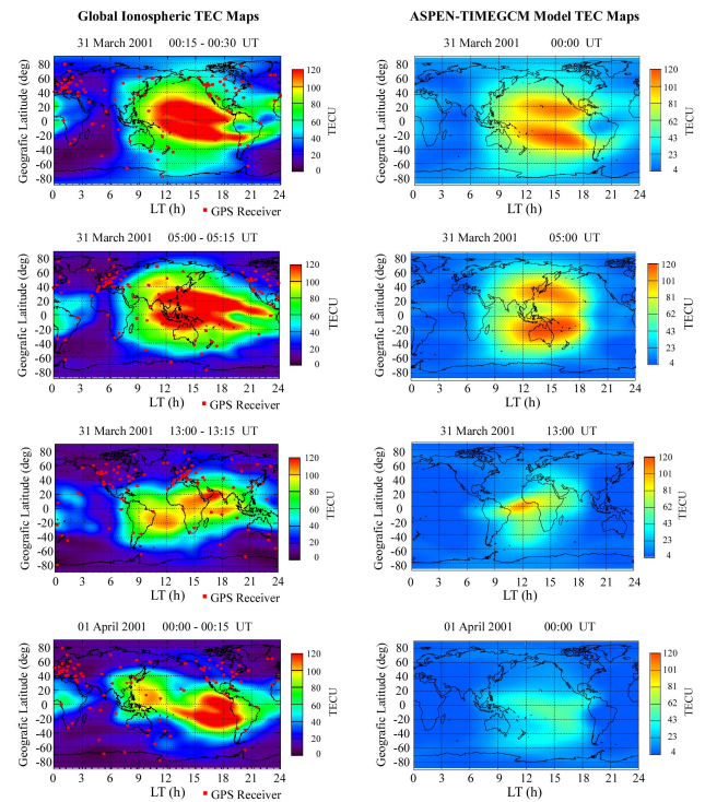
Fig. 5. Global ionospheric TEC maps obtained from GPS network for the time periods 00:15–00:30 UT, 05:00–05:15 UT and 13:00–13:15 UT on 31 March and 00:00–00:15 UT on 1 April 2001. Also, the ASPEN-TIMEGCM model map plots for TEC from 31 March and 1 April are shown.
