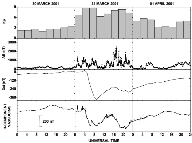
Fig. 1. Time variations of the K_p , AE and D_{st} geomagnetic indices for the period 30 March–1 April 2001. Also, the geomagnetic field H-component variations observed at Vassouras, Brazil are shown.
