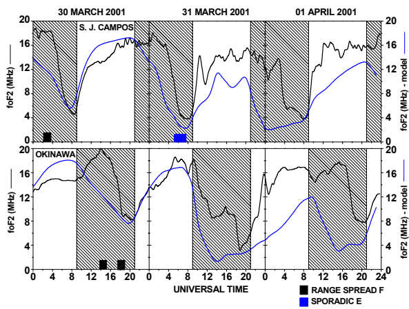
Fig. 2a. F-region critical frequency ( foF2 ) variations (black) observed at low-latitude stations São José dos Campos and Okinawa during the period 30 March–1 April 2001. The hatched portions indicate the local nighttime (18:00–06:00 LT) periods. The black and blue horizontal bars indicate the presence of range spread-F and sporadic E, respectively. Peak F-region critical frequency ( foF2 ) variations obtained from the ASPEN-TIMEGCM model runs are also shown (blue).
