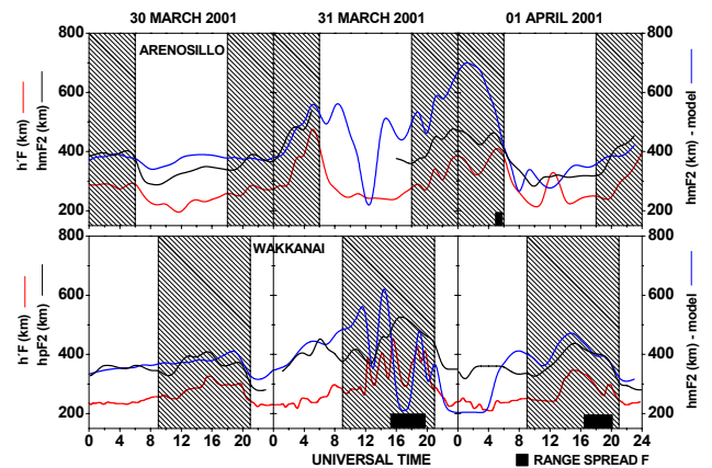
Fig. 4b. Same as in Fig. 2b, but for mid-latitude stations El Arenosillo and Wakkanai, except hmF2 at El Arenosillo.
