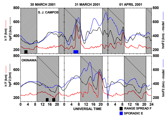
Fig. 2b. F-region minimum virtual height ( h'F – red) and hpF2 (black) variations observed at low-latitude stations São José dos Campos and Okinawa during the period 30 March–1 April 2001. The hatched portions indicate the local nighttime (18:00–06:00 LT) periods. The black and blue horizontal bars indicate the presence of range spread-F and sporadic E, respectively. Peak F-region height ( hmF2 ) variations obtained from the ASPEN-TIMEGCM model runs are also shown (blue).
