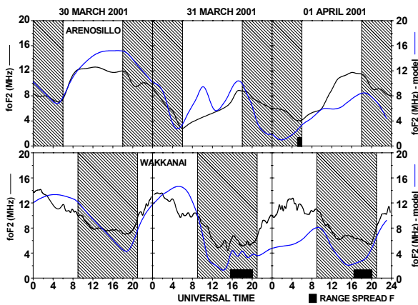
Fig. 4a. Same as in Fig. 2a, but for mid-latitude stations El Arenosillo and Wakkanai.
