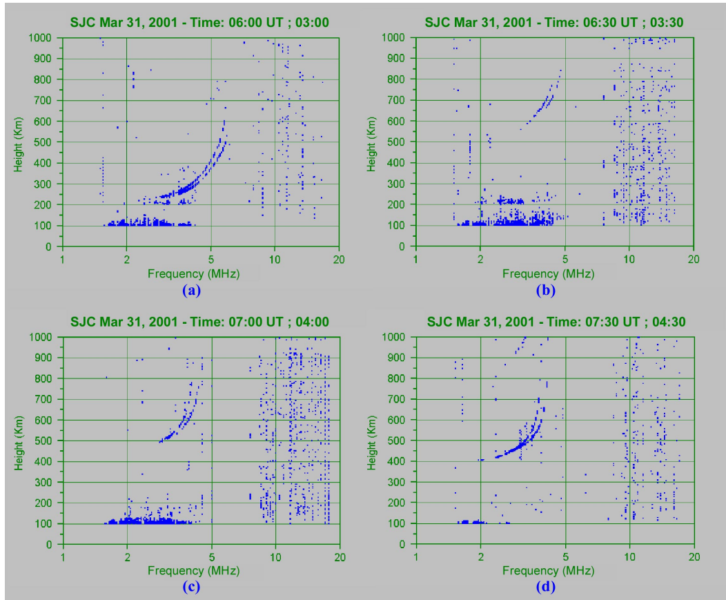
Fig. 3. Ionograms obtained at São José dos Campos between 06:00 and 07:30 UT (03:00–04:30 LT) on 31 March showing the presence of intense sporadic E at the time of the unusual uplifting of the F-region.
