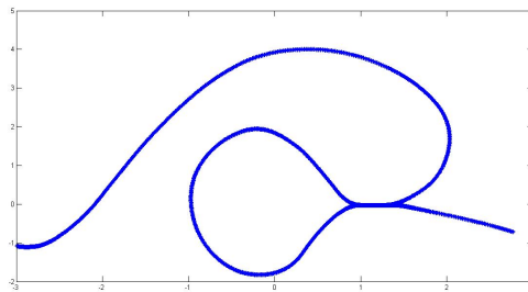
Figure 2: A splat singularity: regular curve with self-intersection along an arc.
