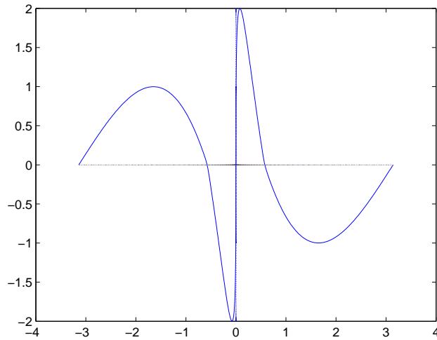
Figure 1: An example of wave-turning for Muskat. At (x, y) = (0, 0) the slope of the function is +\infty .
