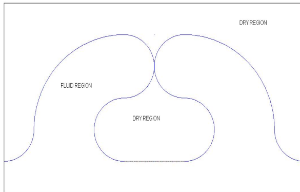
Figure 3: An appropriate geometry for a splash singularity in Muskat with a dry region.
