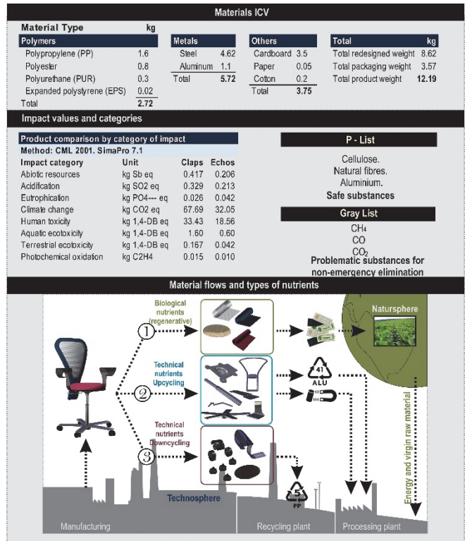
Figure 6 Summary of life cycle analysis and criteria for C2C certification of the product; Source: The authors
