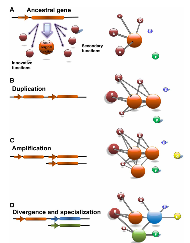
FIGURE 5 | The Innovation-Amplification-Divergence (IAD) model of evolution by gene duplication explains the evolutionary history of the CrCO , PpCOL , and AtCOL genes. (A) The CrCO gene in Chlamydomonas is a hub gene whose main functions are light response and carbon/nitrogen metabolism. Additionally, CrCO presents links to secondary functions such as response to chemical stimulus and developmental processes that can be considered innovations developed by this gene. (B) During the evolution of multicellular land-based plants such as Physcomitrella and Arabidopsis these secondary functions became selectively valuable which facilitated the fixation of duplications of CrCO . Initially, duplicated genes are identical and conserved exactly the same links as the ancestral gene. (C) In order to fully cover the demands exerted by selection of a more complex regulation over developmental processes, an amplification consisting of multiple gene duplications took place, giving rise to the 10 gene family of PpCOLs and the 17 gene family of AtCOLs . (D) After duplication and amplification the same selective forces facilitate the accumulation of mutations over the duplicated genes that make them diverge, specialize and acquire new functions as it can be observed in the PpCOL and AtCOL genes. This is reflected in the network by the removal of links and the establishment of new ones. Note that in spite of divergence the genes tend to keep links to the main ancestral functions.
