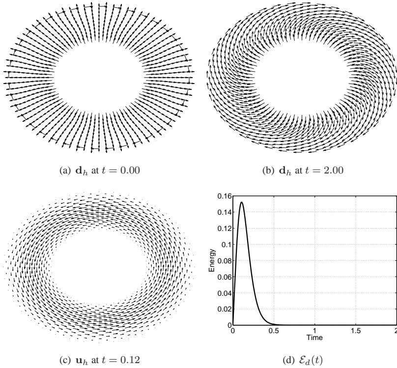
FIG. 6.10. Example 2: Director vector \mathbf{d} fields at different time step values, velocity vector field and \mathcal{E}_d(t) plot for the nodal implicit method with \epsilon = 0 .
