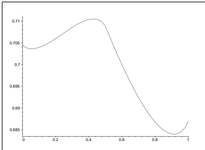
Figure 1: Objective function H_{12}(x) in Example 1
