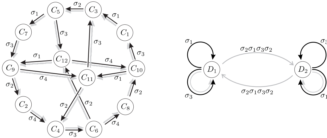
Figure 3: \Gamma_C and \Gamma_D .
