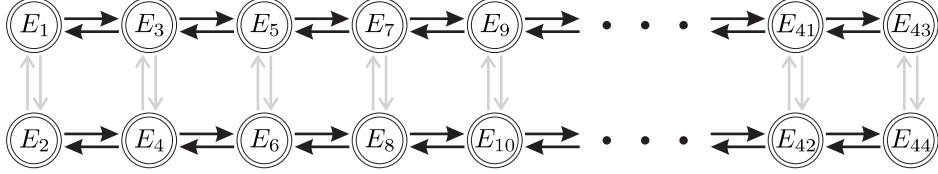
Figure 4: The quotient graph \Gamma_E/\phi illustrates a very long path of iterated partial cyclings.
