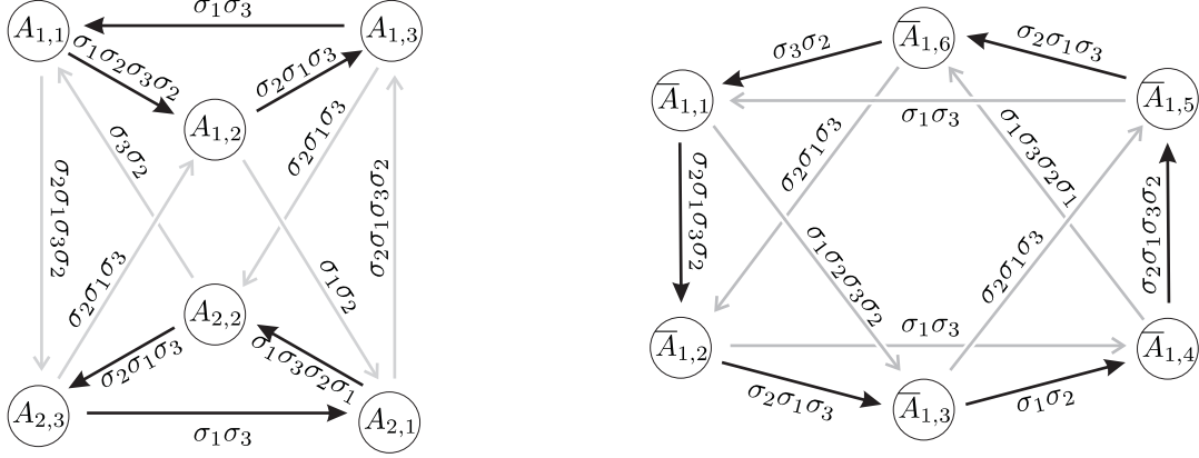
Figure 1: The graphs \Gamma_A and \Gamma_{\bar{A}} = \Gamma_{A^{-1}} .
