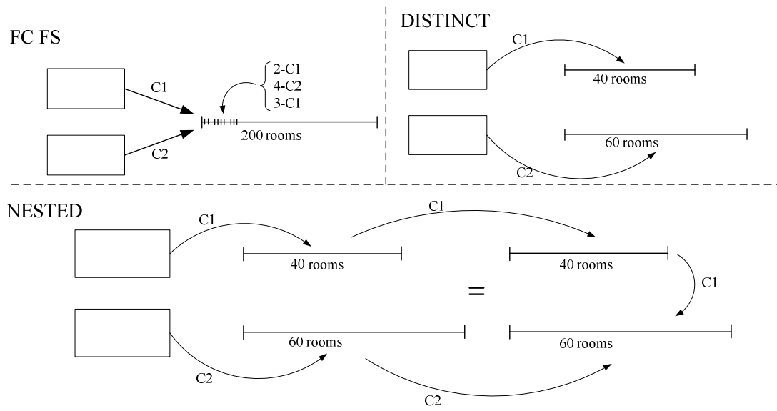
Figure 3 Heuristics of room inventory control
