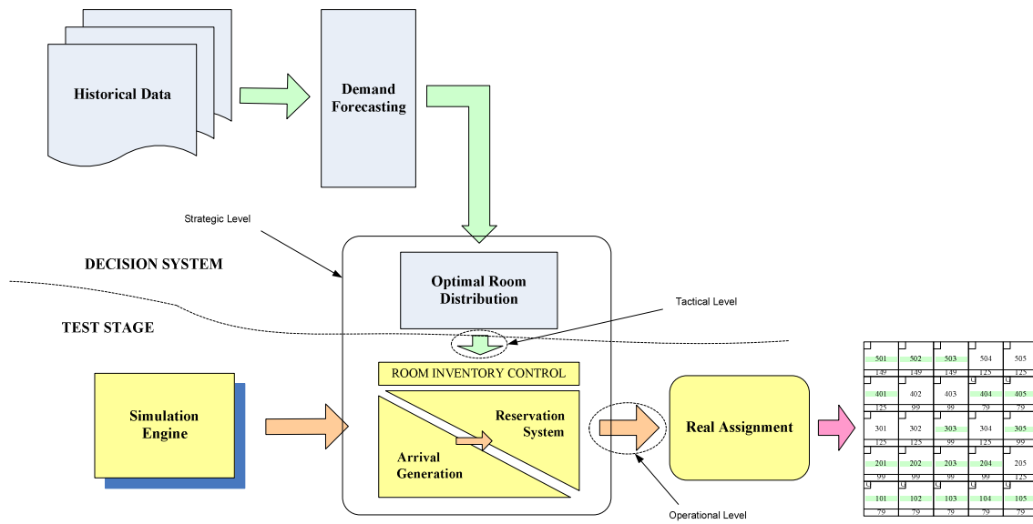
Figure 1 Decision Support Revenue Management System process flow
